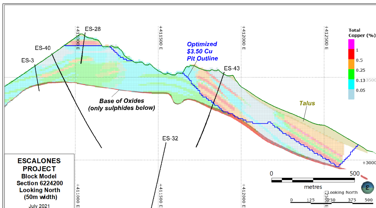
Figure 1: East-west Cross Section of the Escalones Block Model at 4200mN, with US$3.50/lb Cu pit shell.
