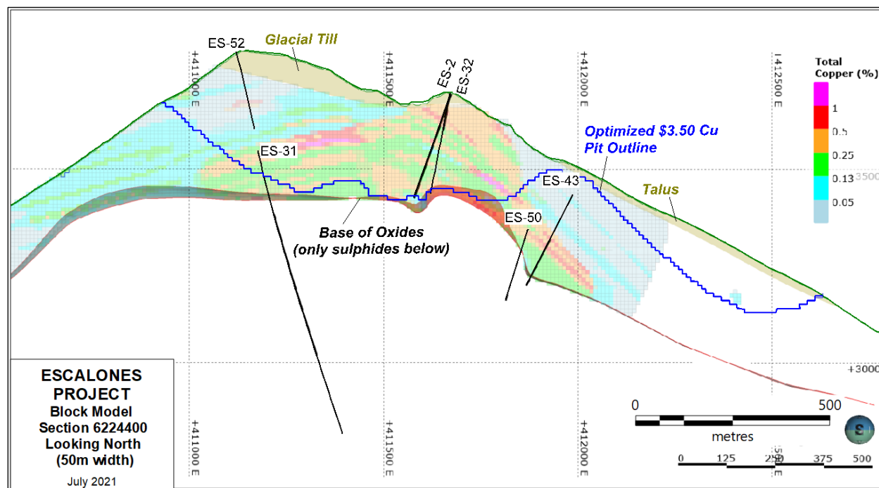
Figure 2: East-west Cross Section of the Escalones Block Model at 4400mN, with US$3.50/lb Cu pit shell.
