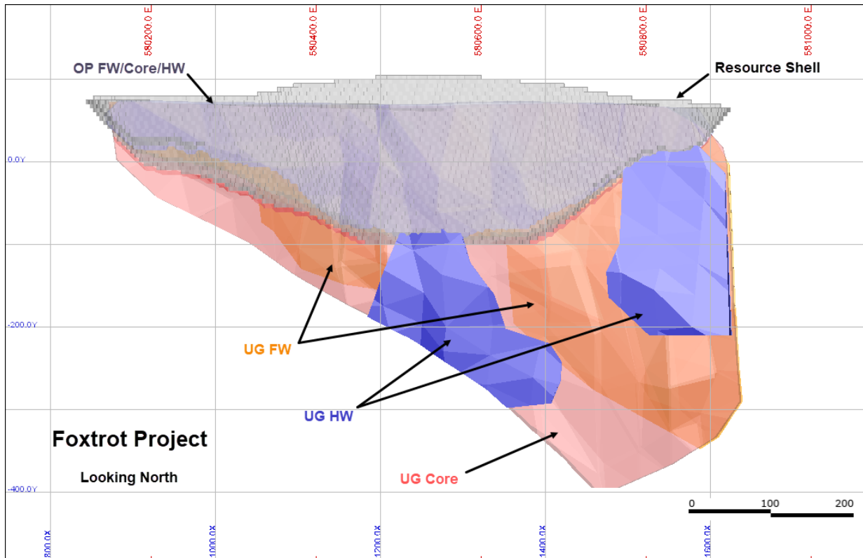
FIGURE 2 Foxtrot Resource Wireframes and Resource Shell
