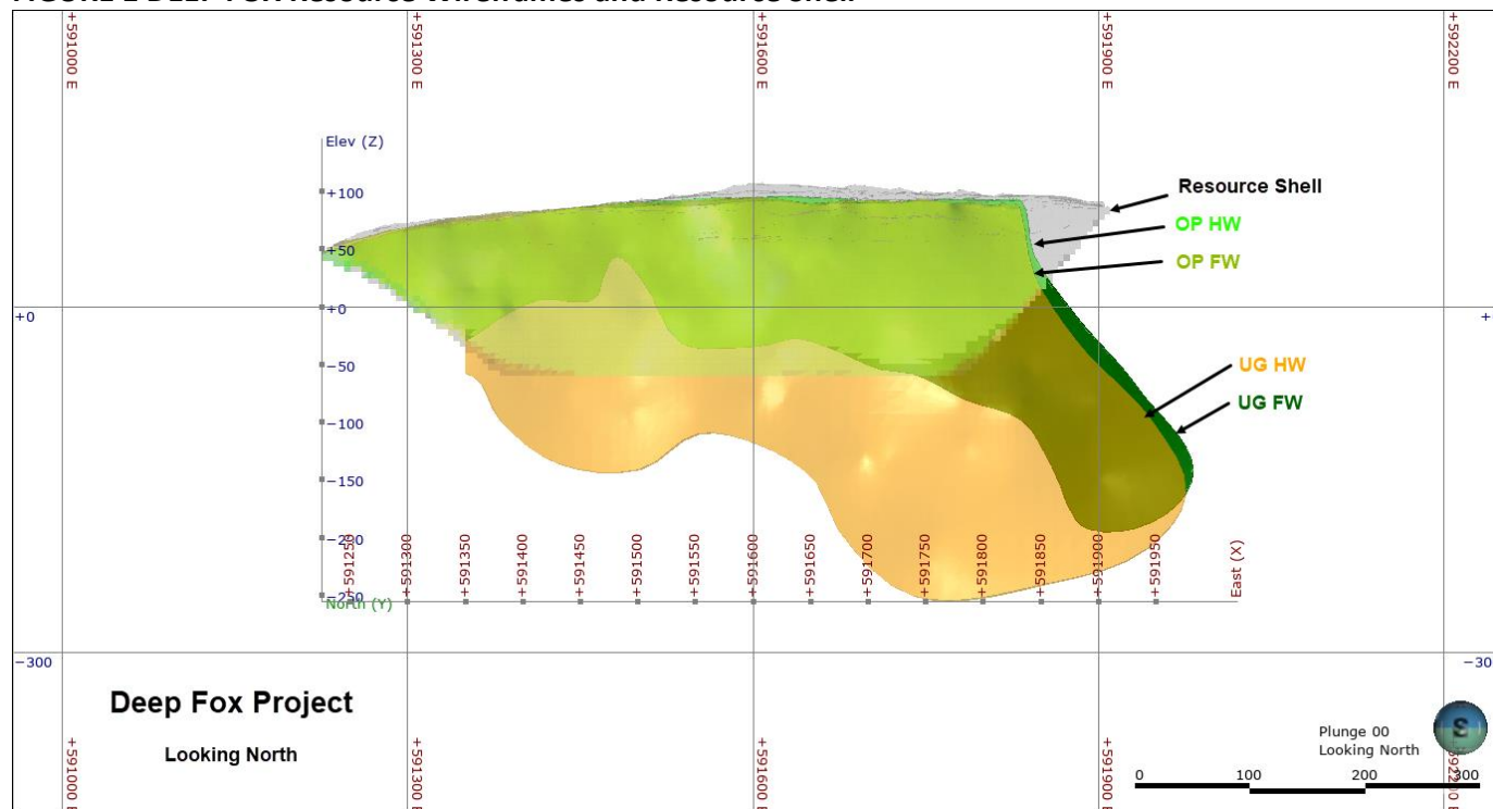
FIGURE 1 DEEP FOX Resource Wireframes and Resource Shell
