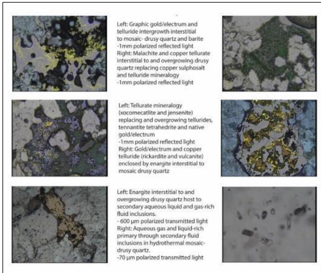
Figure 8.7 Thin Sections from the T2 Structure
