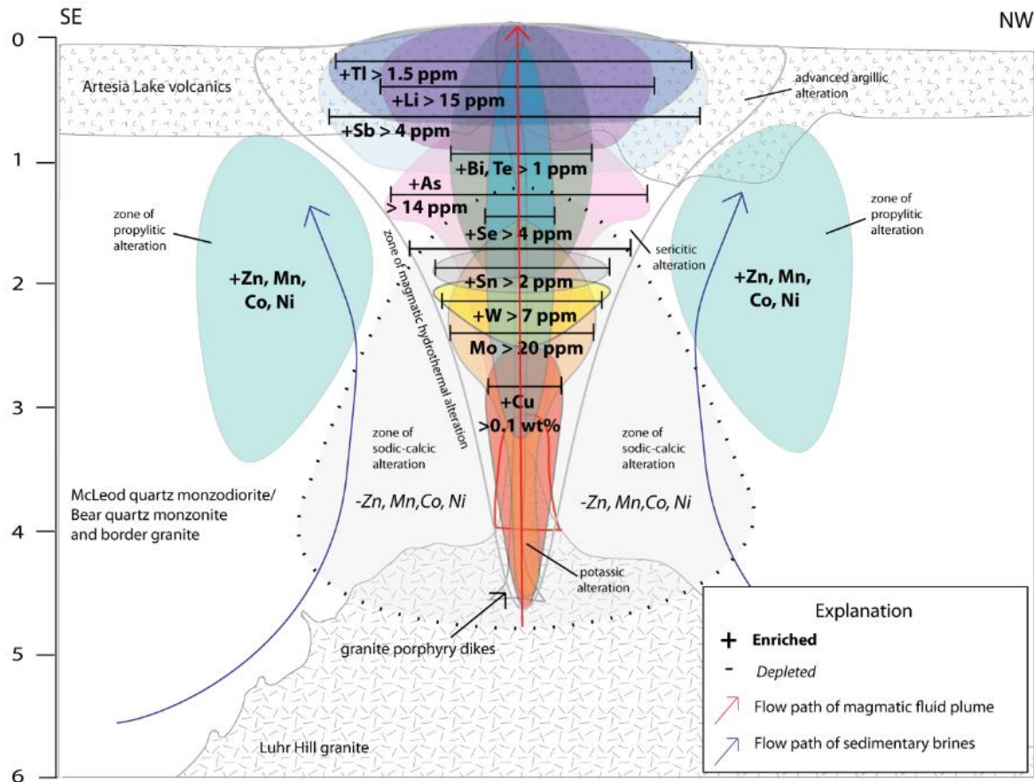
Figure 9.17 From Cohen (2011) Showing the Relative Position and Scale of Geochemical Variations Associated with the Ann Mason Porphyry Copper Deposit, Nevada.
