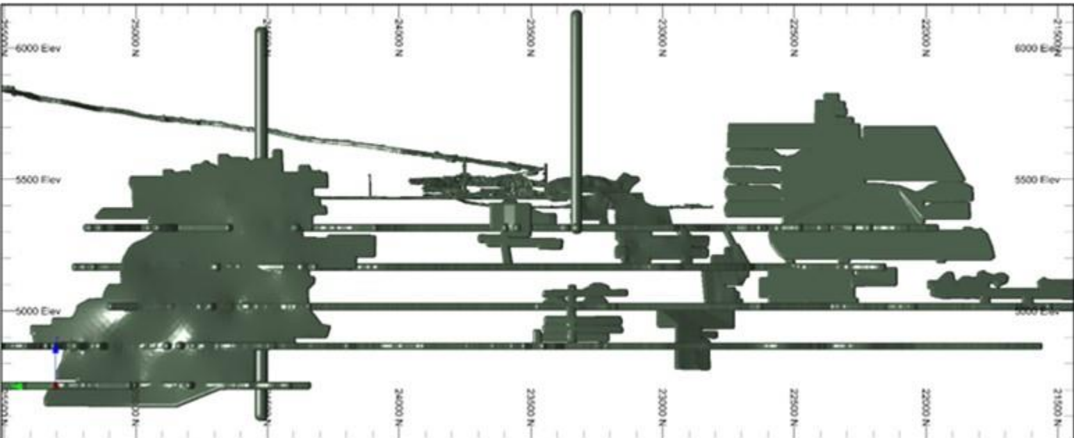
Figure 14.6 Vertical Long Section Looking East at the Current Development Voids and Historical Buffers, Used to Deplete the Trixie Mineral Resources
