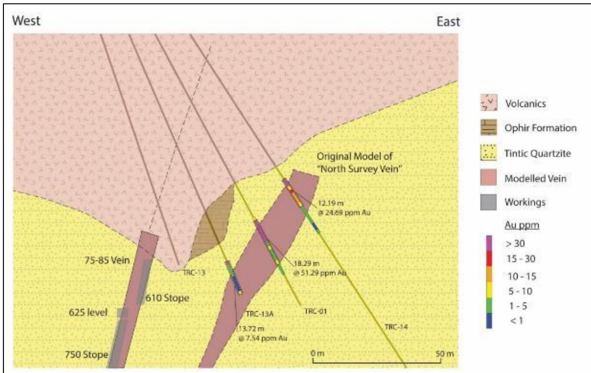
Figure 6.3 Cross-Section, Looking North, of the Surface RC Hole Intersections that Led to Discovery of the T2 Structure
