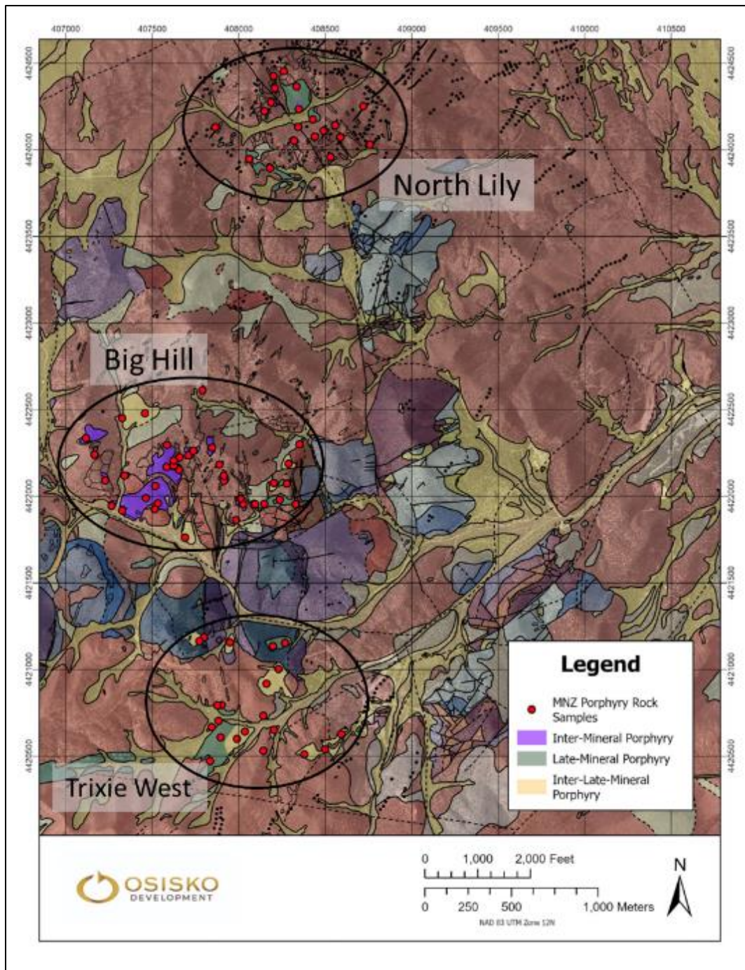
Figure 9.16 Location Map of Porphyry Samples and Subdivision of Intrusive Centres Used for Analysis
