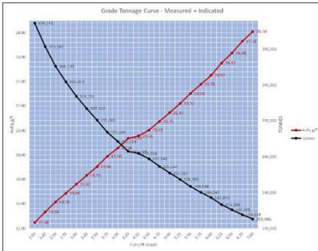
Figure 14.7 Grade Tonnage Curves Indicating the Sensitivity of the Measured and Indicated Mineral Resources at Different Cut-Off Grades
