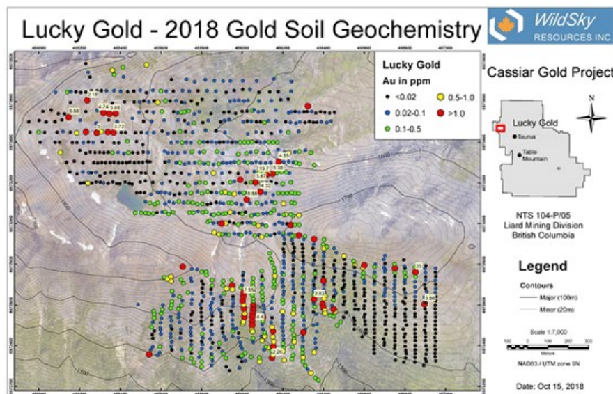
WildSky Resources - 2018 Gold in Soil Geochemical Map
