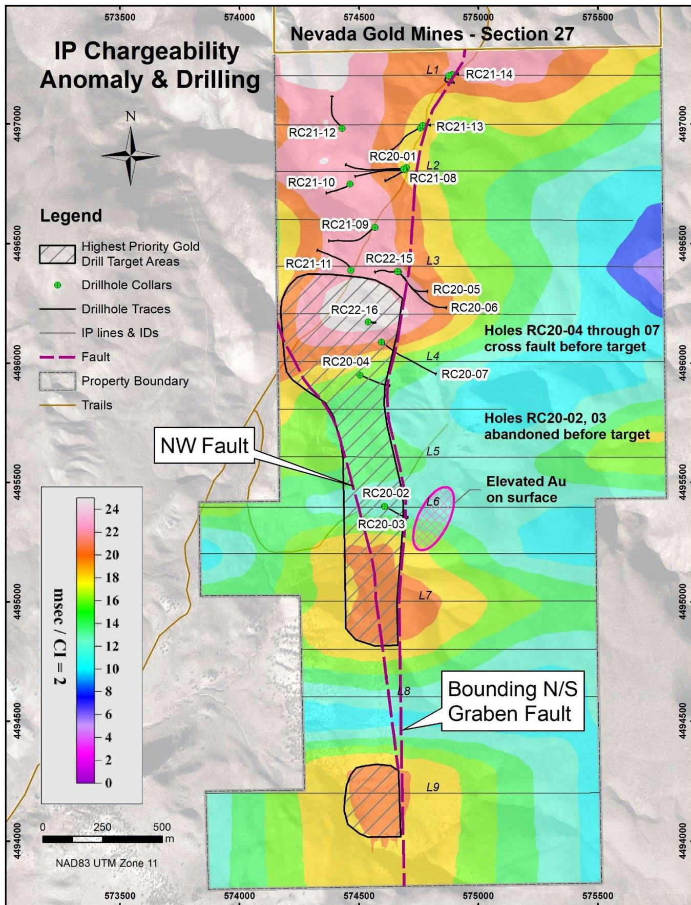
Figure 1: Gold Target Drilling to Date on Carlin Gold-Vanadium Project and its Highest Priority Untested Areas
