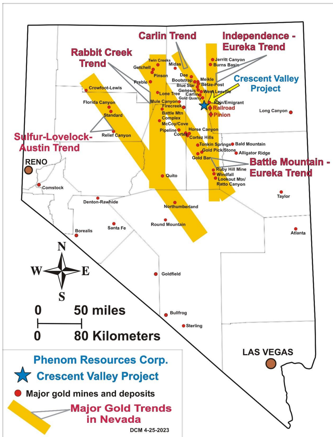
Figure 1: Principal Gold Trends in Nevada and Location of Crescent Valley Project
