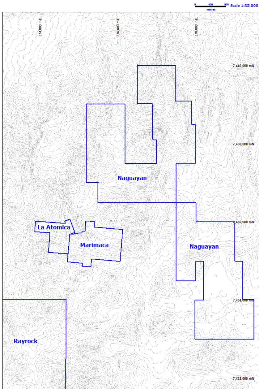
Figure 2: Naguayan Claims together with Coro's Marimaca, La Atomica & Rayrock Claim Blocks
