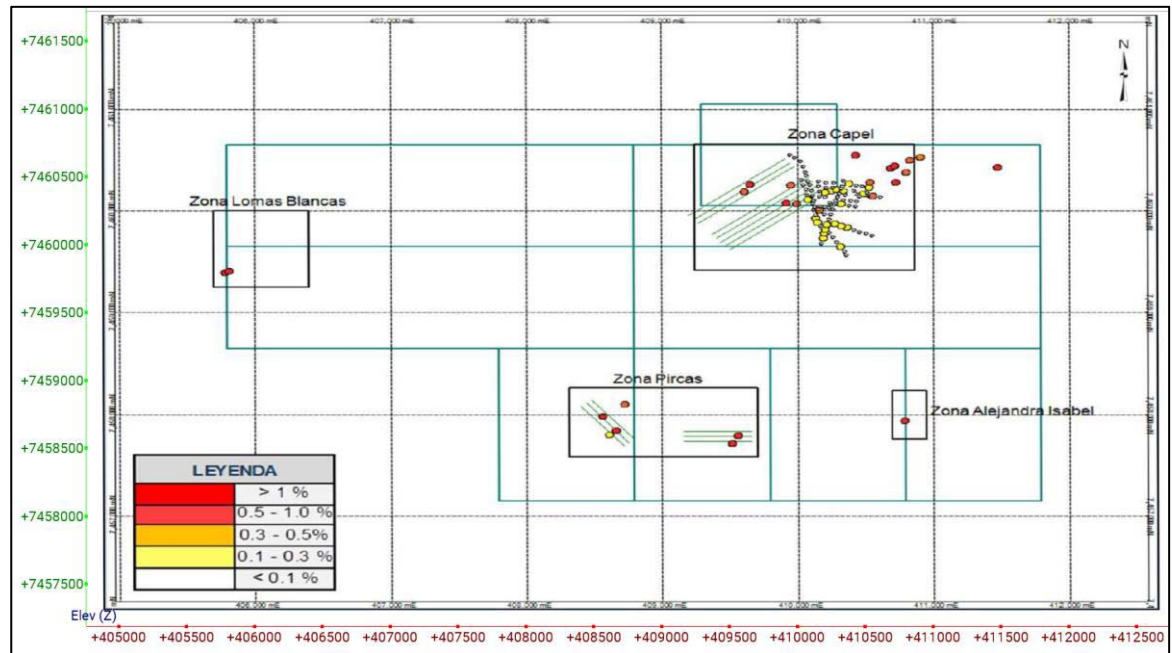
Figure 5.2: Antennas sub-areas and geochemical copper anomalies
