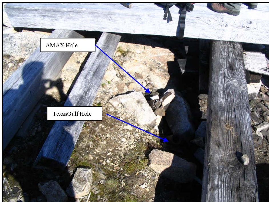
Twinned Drill Holes
