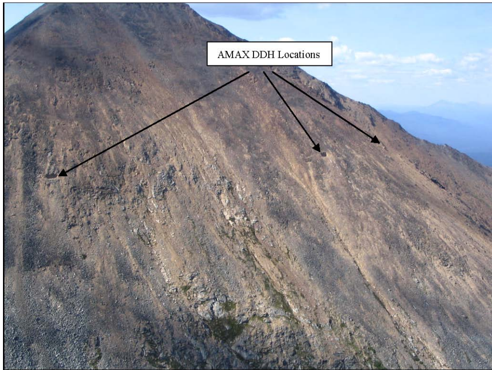
AMAX Drill Hole Locations
