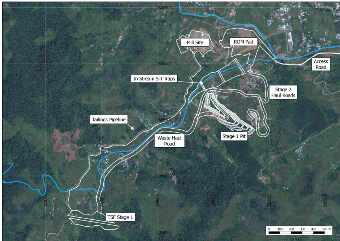
Figure 16.1: Stage 1 Open Pit
