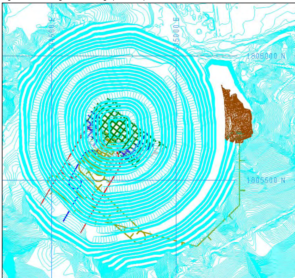
Figure 16.6: Underground Workings (Plan View)
