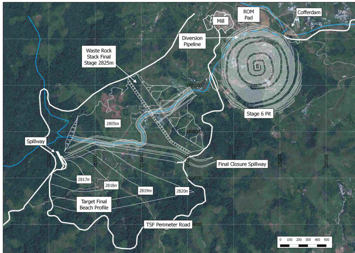
Figure 16.4: Stage 6 Open Pit (Final)
