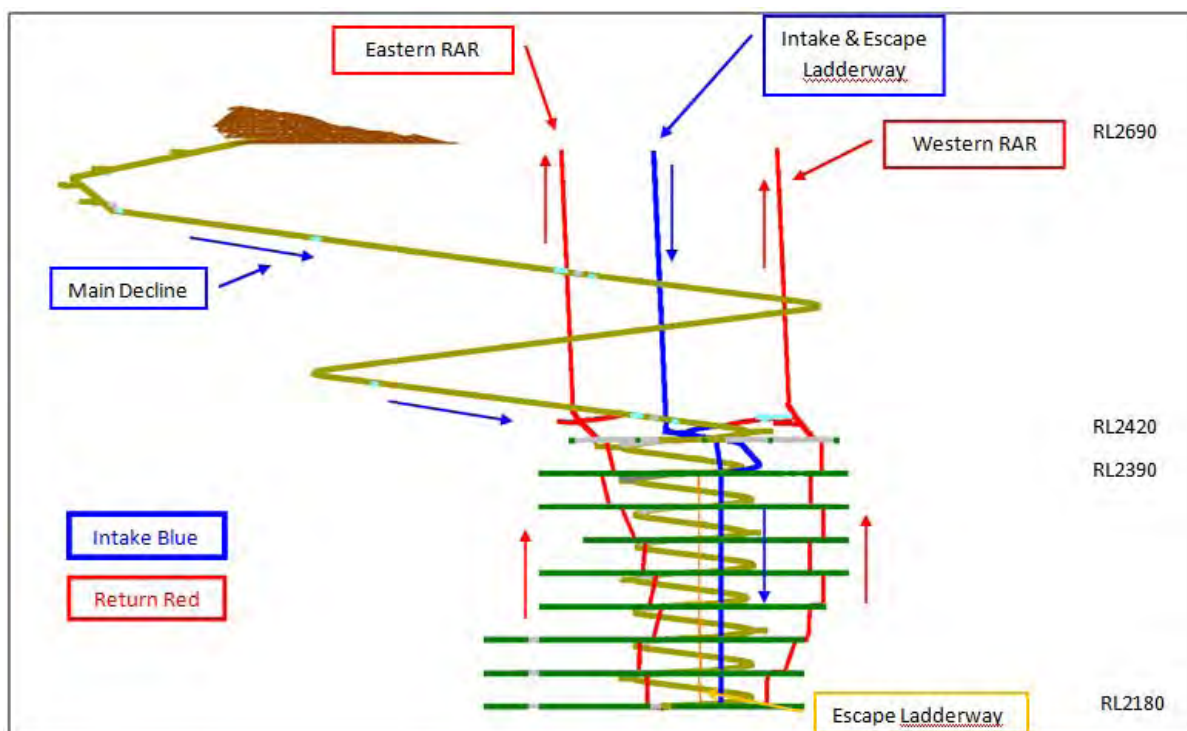
Figure 16.11: Ventilation Network
