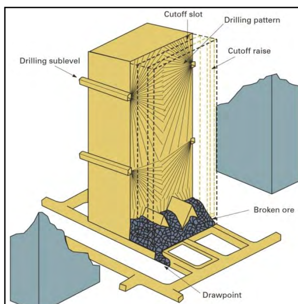
Figure 16.12: Sub-Level Open Stopping Method (Schematic Section)
