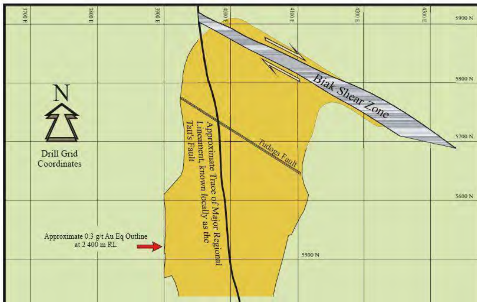
Figure 7.8: Approximate Location of Major Structures (2400mRL)
