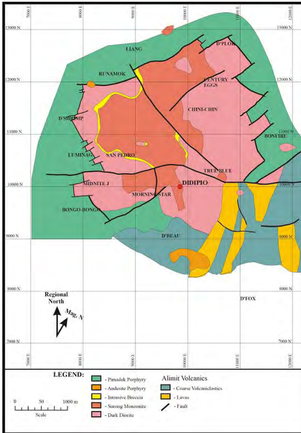
Figure 7.3: Local Geology
