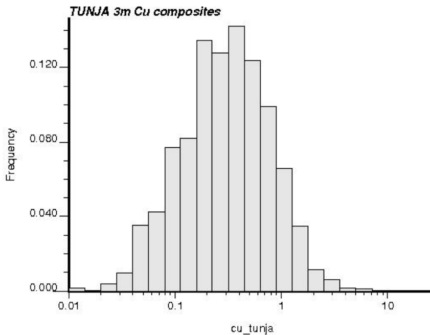
Figure 14.3: Histogram of 3m Composited Copper Grades for Tunja Monzodiorite
