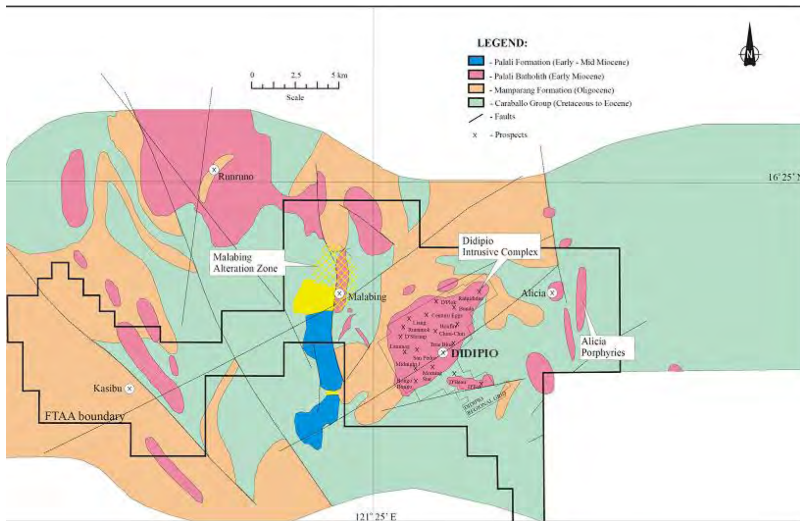
Figure 7.2: Regional Geology
