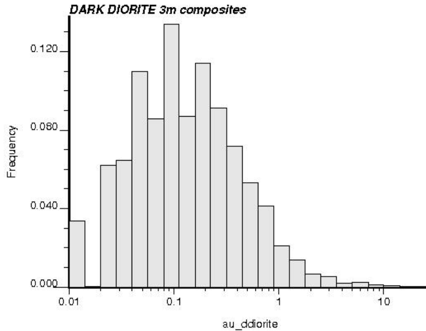
Figure 14.2: Histogram of 3m Composited Gold Grades for Dark Diorite
