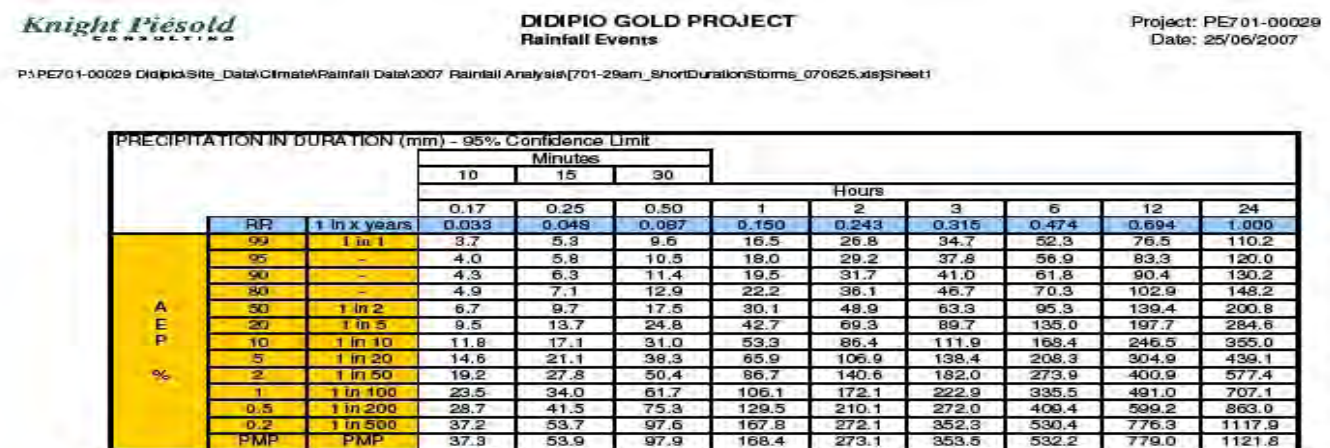
Figure 5.3: Rainfall Modelling
