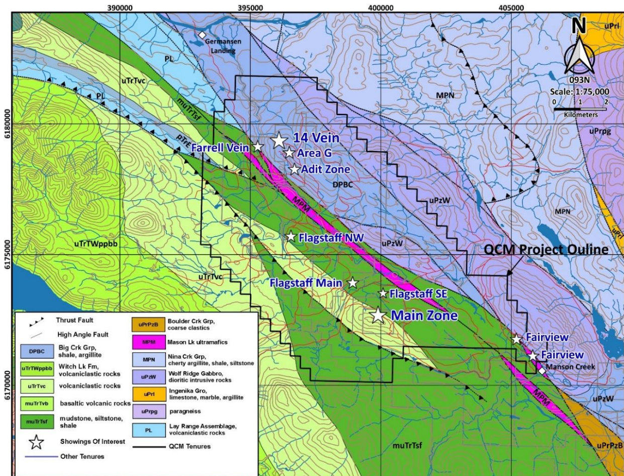
Figure 2: Property Outline with Showings on Geology
