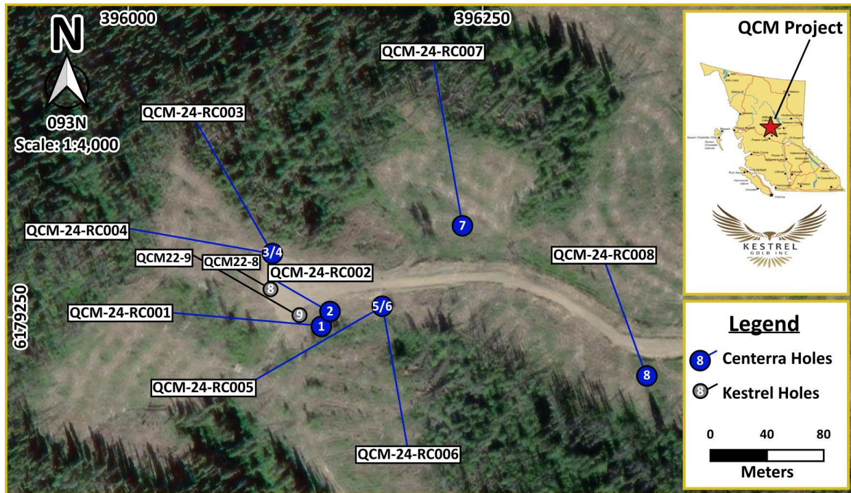
Figure 1: 14 Vein Zone, Hole Locations on Imagery
