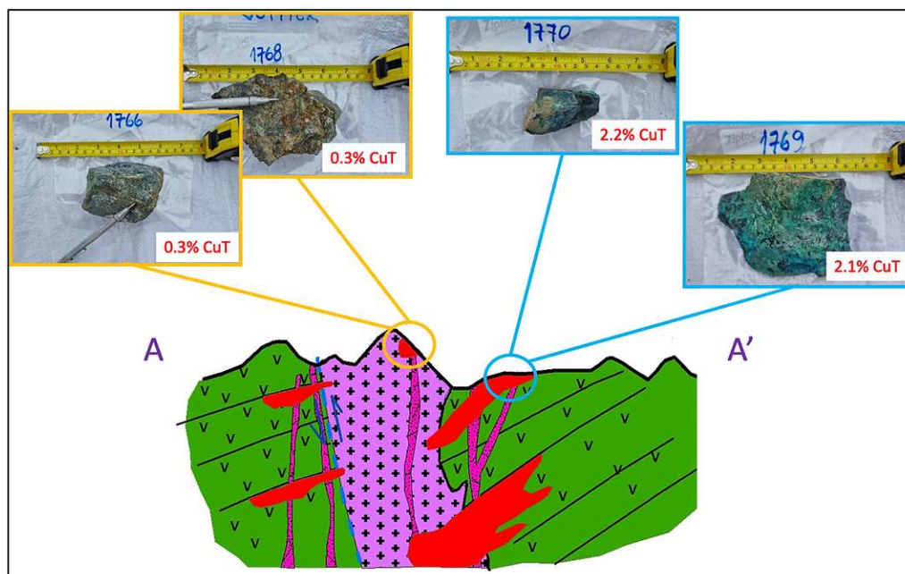
Figure 4 - Interpretation of cross section A-A'
