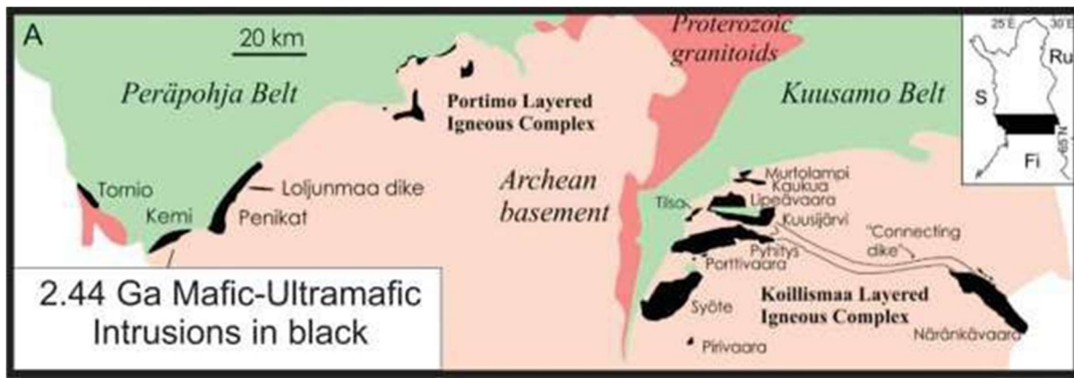
Figure 7-2 – Simplified geology of the Tornio Näränkävää intrusion belt (TNB), showing the Kemi Intrusion, host to the world class Kemi chrome mine, the Portimo Complex host to the Suhanko PGE-Ni-Cu deposit, and the Koillismaa Complex which hosts the LK Project
