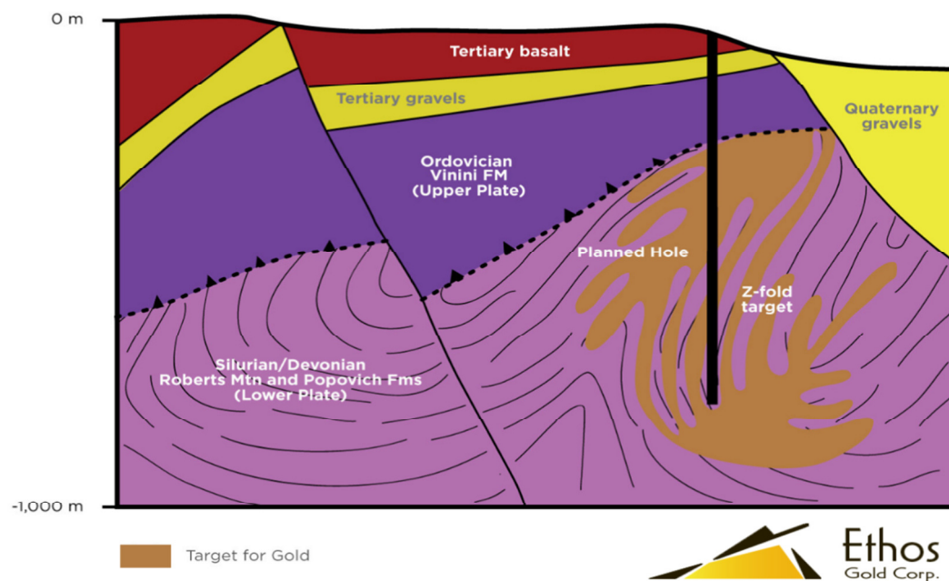
Figure 4. Conceptual east-west cross section B-B' (see section line on Figure 2)
