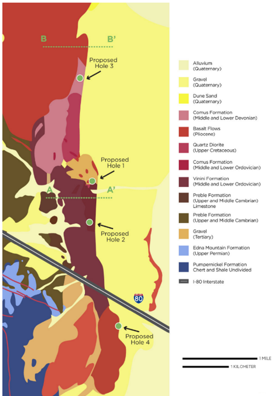
Figure 2. Geology in plan and location of the 4 planned holes, also showing East-West section lines A-A' and B-B'
