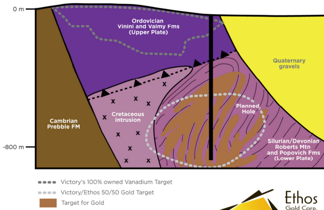
Figure 3. Conceptual east-west cross section A-A' (see section line on Figure 2)
