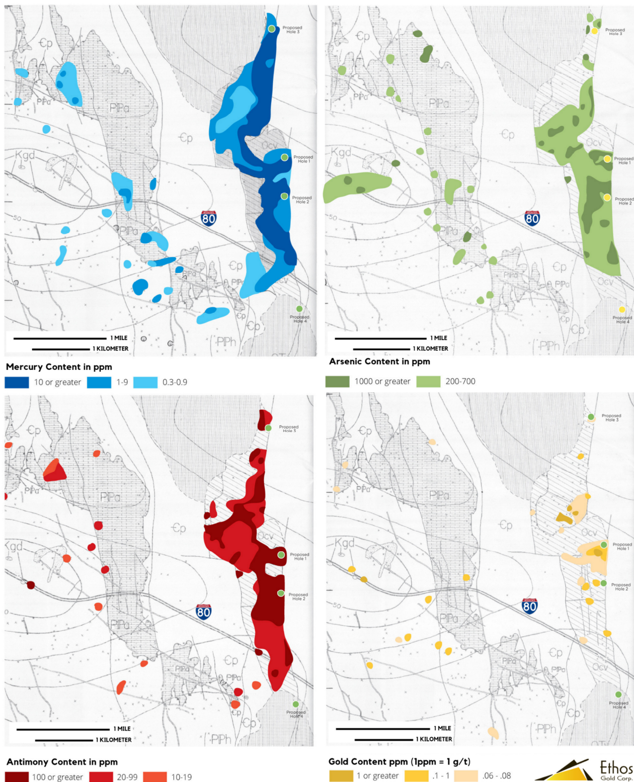
Figure 5. Iron Point surface geochemistry along the range front fault, also showing planned drill hole locations
