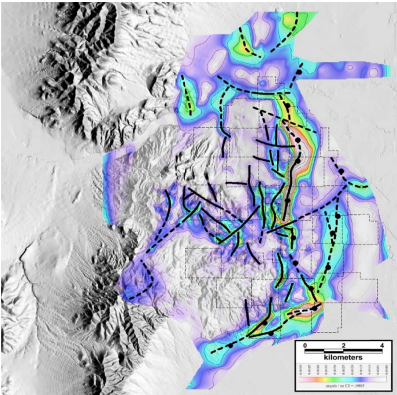
Figure 5. Total Field Residual Gravity with structural interpretation at Iron Point, NV.
