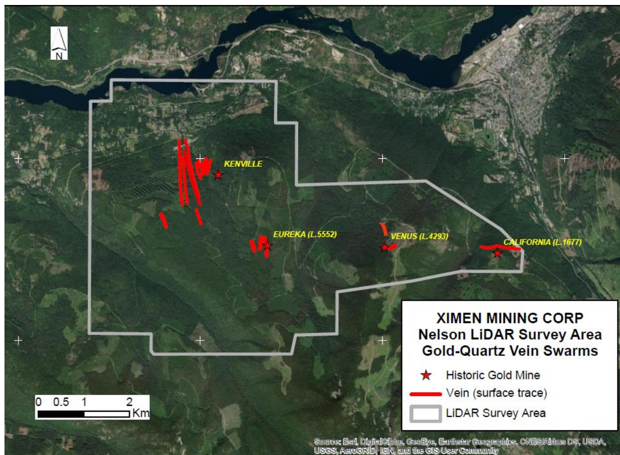
Figure 2. Map of known vein swarms extending over 8 x 3 km area within LiDAR survey area..
