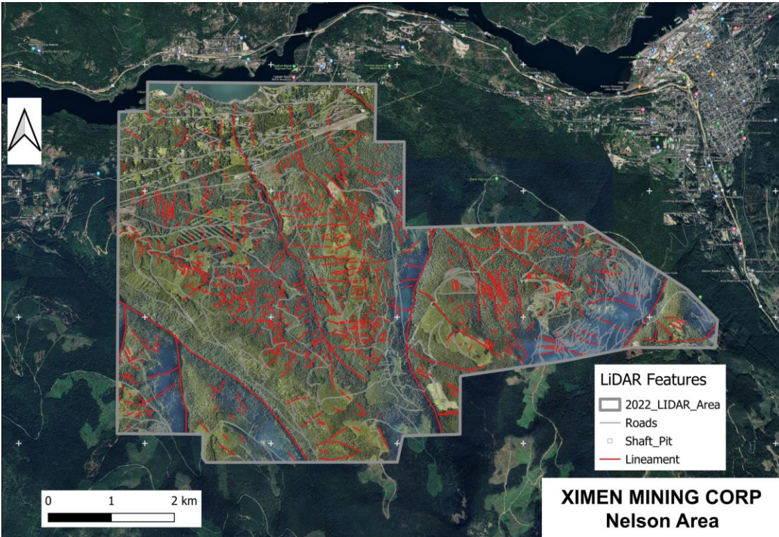
Figure 4. Image of the orthomosaic from the LiDAR survey showing lineaments identified.
