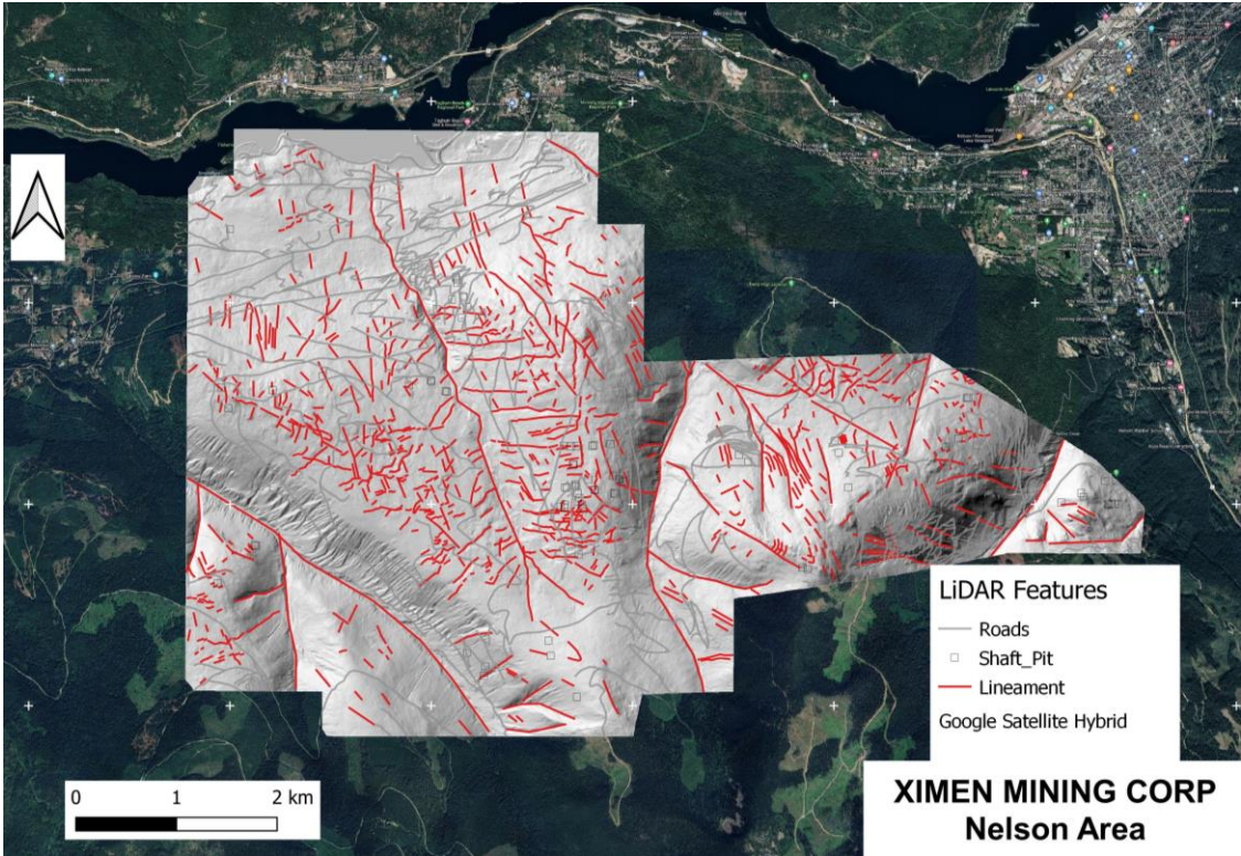
Figure 3. Lineaments identified from LiDAR DEM.
