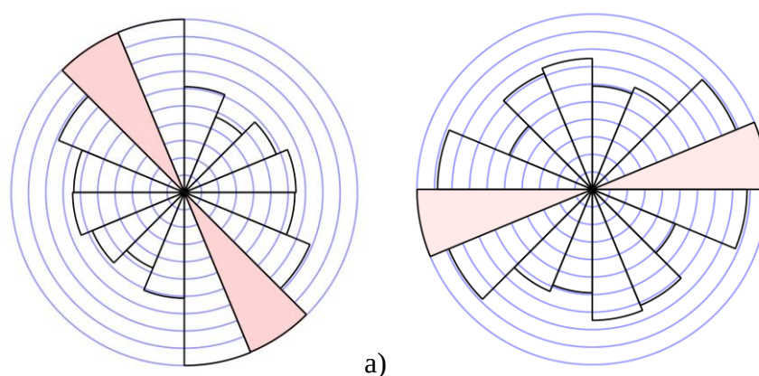
Figure 4. Rose diagrams of lineaments showing length-weighted (a) and non length-weighted groupings (b).
