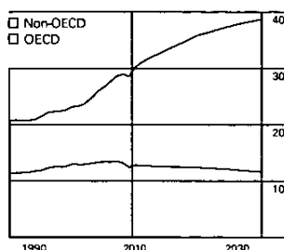
Global CO 2 emissions from energy use by region (billion tonnes CO 2 )
