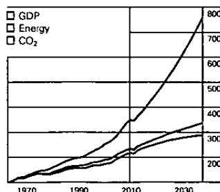
Global CO 2 emissions from energy use vs GDP and energy (Index 1970 = 100)
