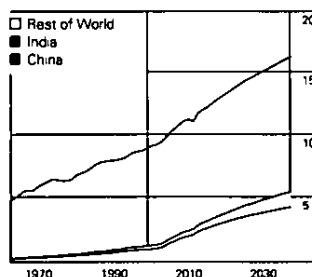
Energy (billion tonnes of oil equivalent)
