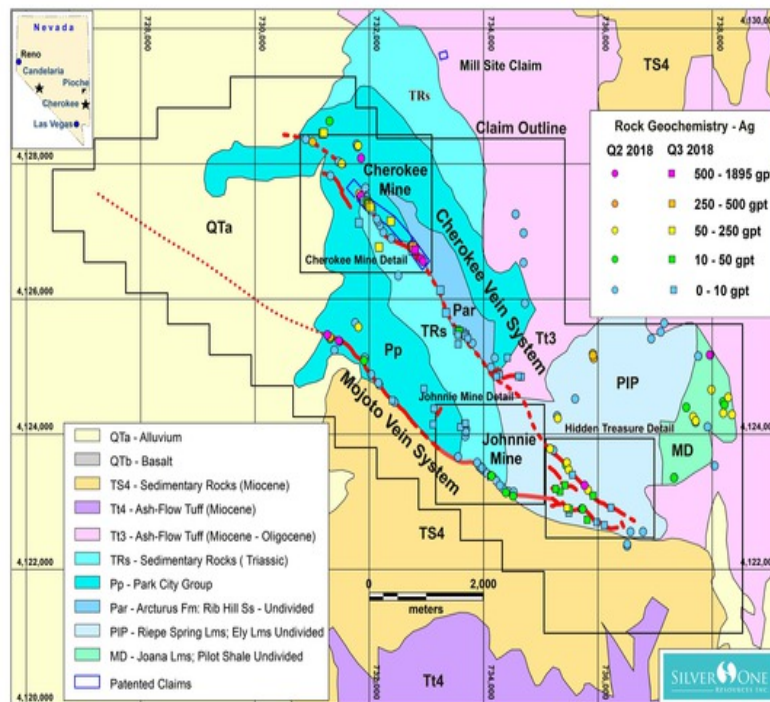
Figure 2: Cherokee-Mojoto-Johnny- Hidden Treasure Vein Systems Silver Geochemistry
