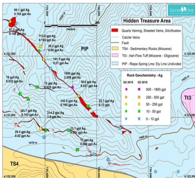
Figure 1: Hidden Treasure Silver Geochemistry and Geology - Topography
