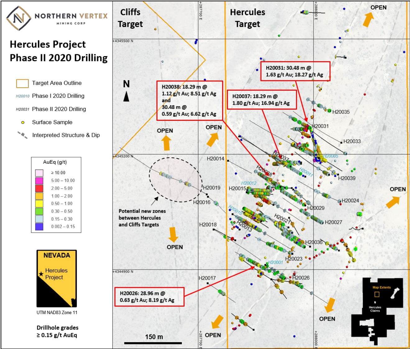
Figure 1. Plan view of Hercules target drilling.
