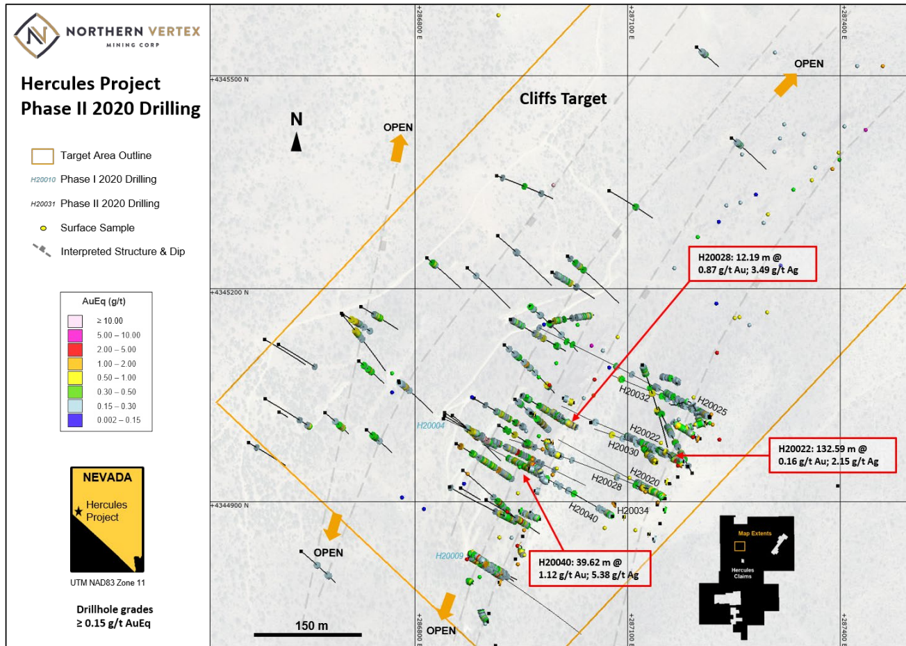
Figure 2. Plan view of Cliffs target drilling
