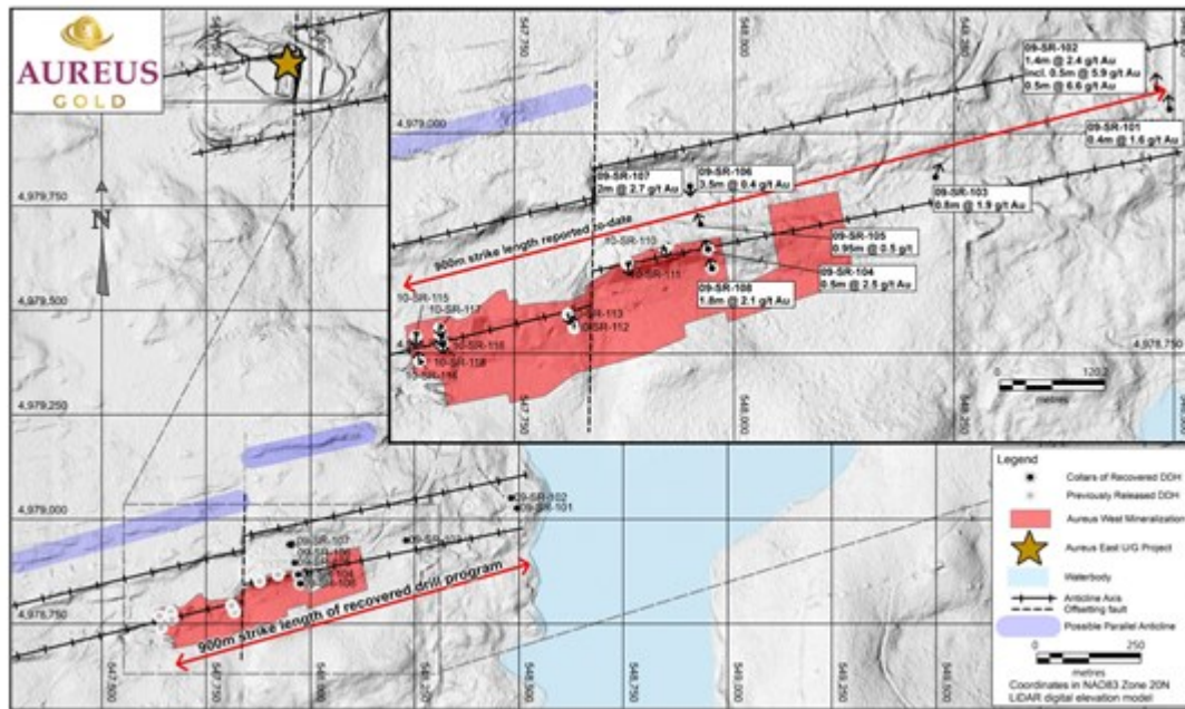
Figure 2: Plan map of Aureus West Project area showing known gold mineralization and drilling on top of Lidar imagery
