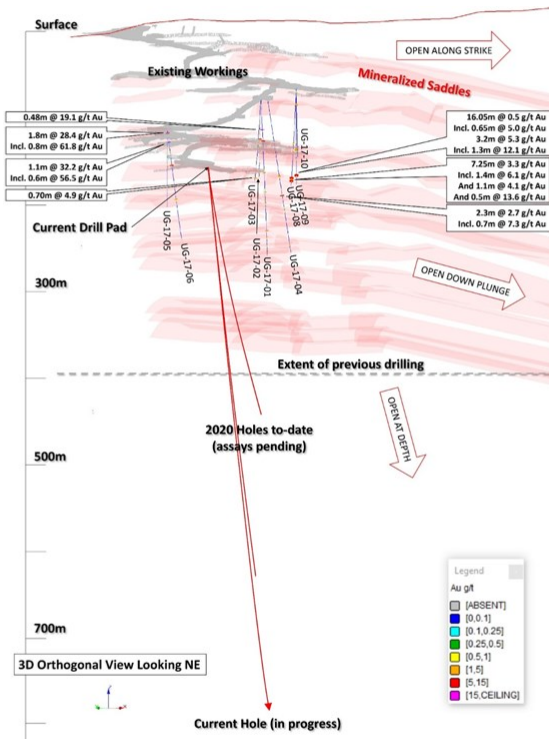
Figure 1: Aureus East orthogonal section showing current drill hole traces and reported holes UG-17-01 to UG-17-10 with gold intercepts, mineralized saddle reef veins and existing underground workings
