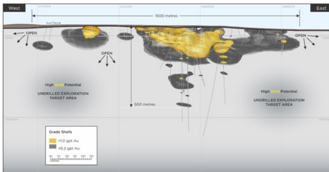
Aureus West Longitudinal Section: Grade Shells Looking North
