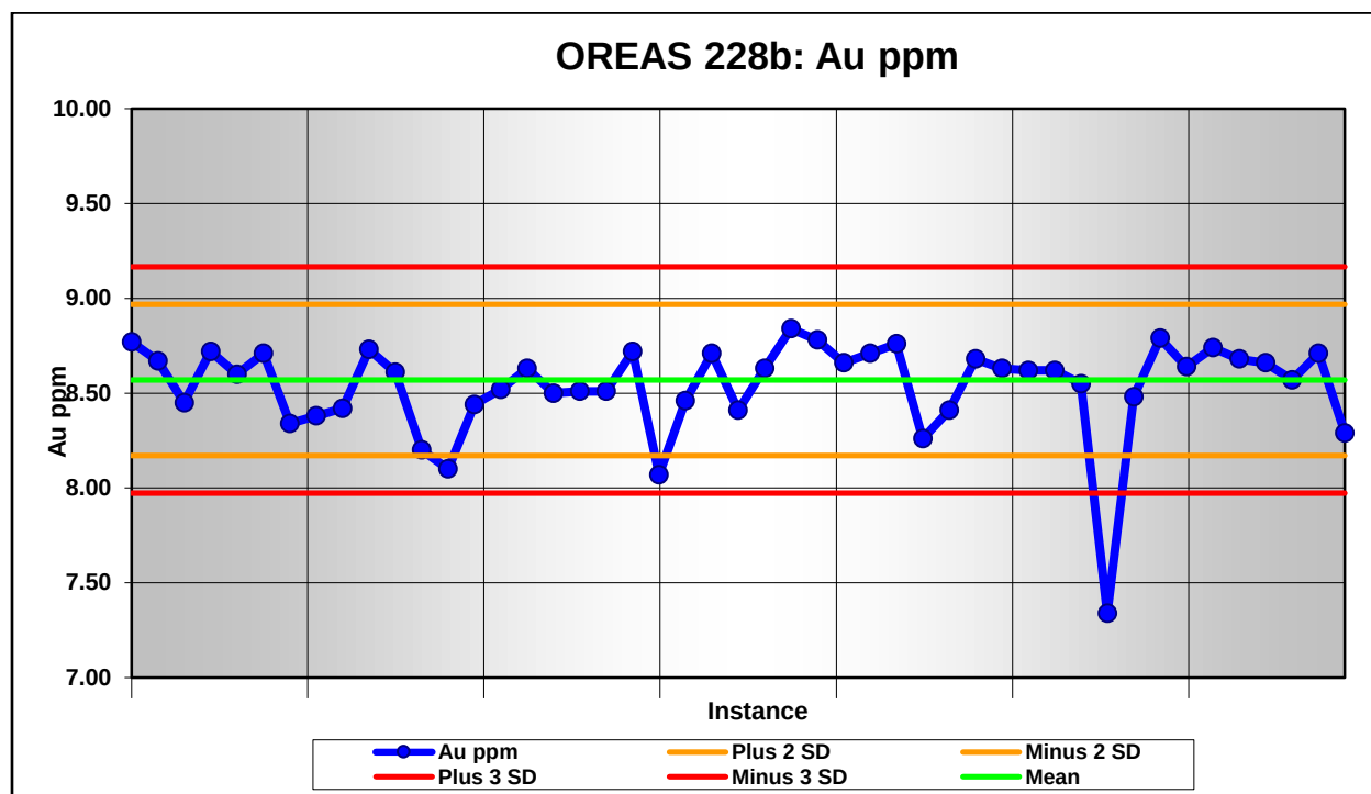
Figure 11-7 CMO Property Control chart for standard OREAS 228b
