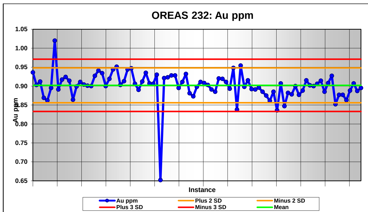
Figure 11-8 CMO Property Control chart for standard OREAS 232
