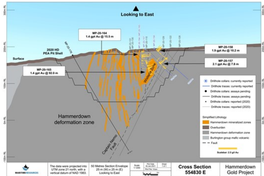
Figure 4: Cross Section 554830 E ( click image to enlarge )
