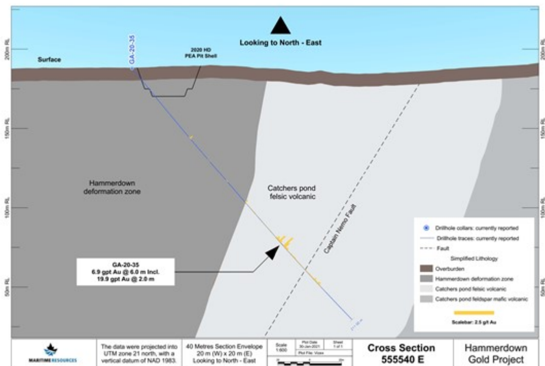
Figure 3: Cross Section 555540 E ( click image to enlarge )
