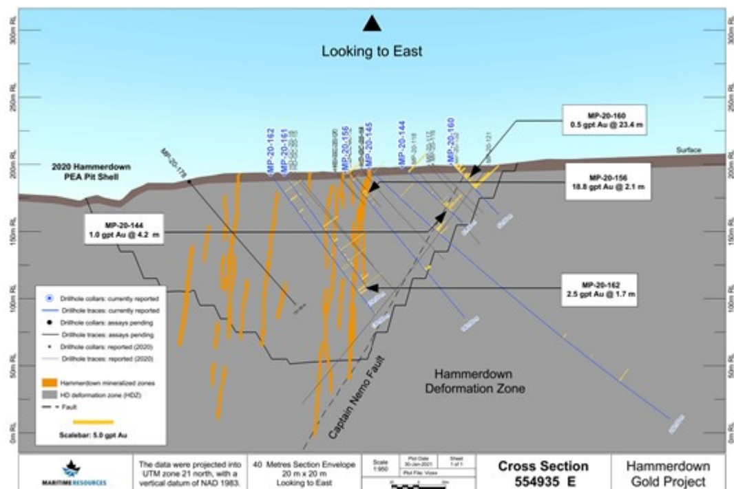
Figure 5: Cross Section 554935 E ( click image to enlarge )
