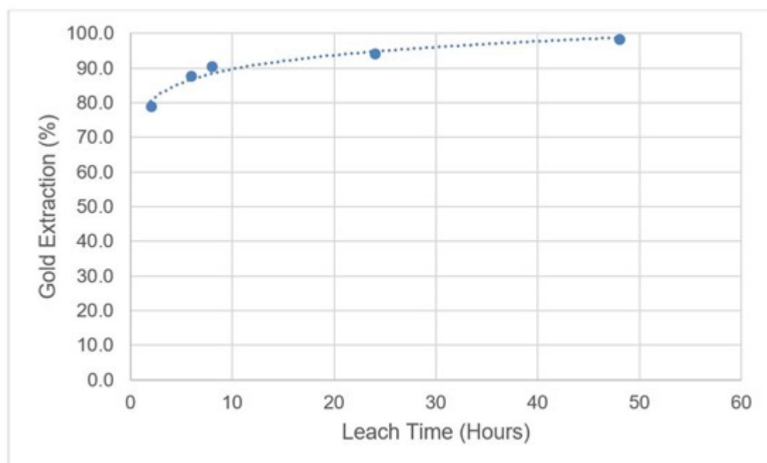
Figure 2. Leach Kinetics
