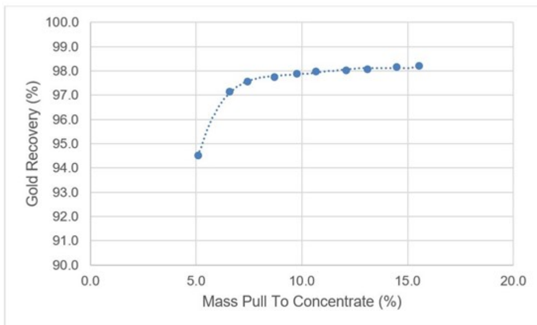
Figure 1. Flotation Mass-Recovery Curve at ~75 µm P80 Grind Size
