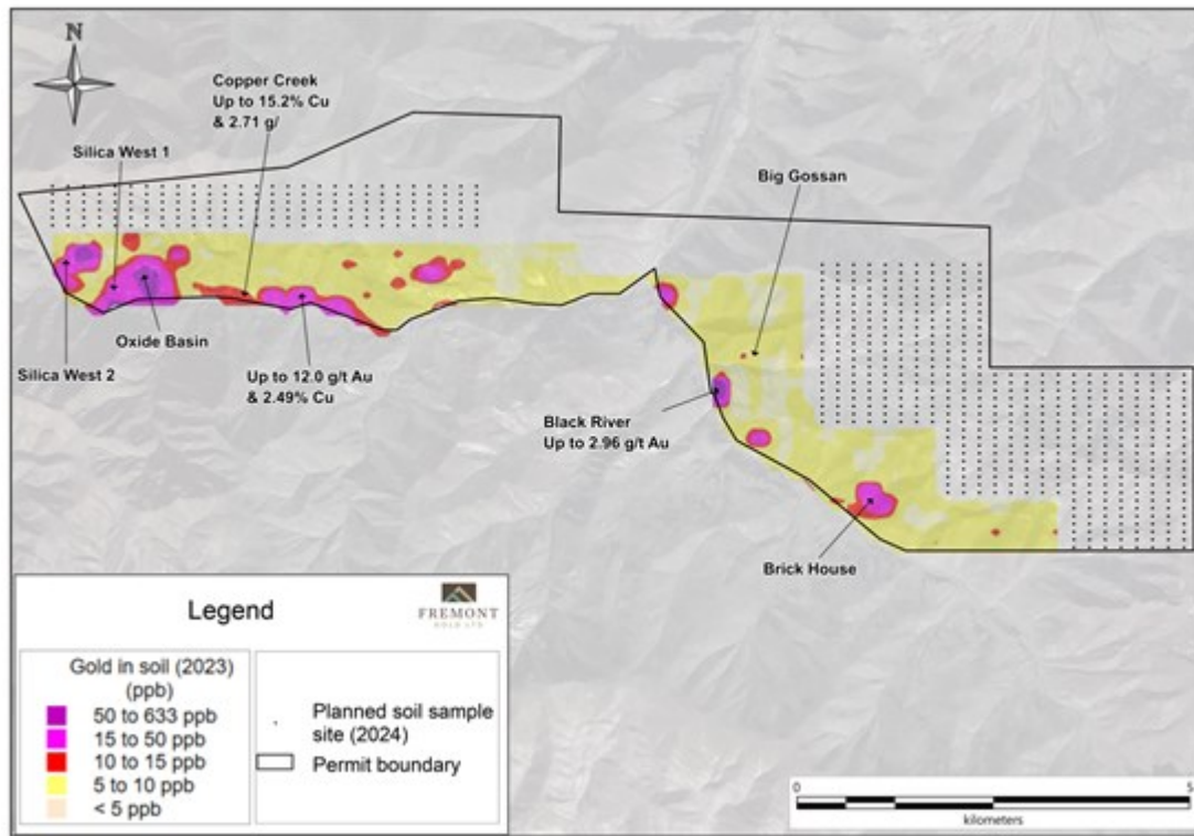
Figure 1. Urasar key target areas, soil and rock geochemistry.
