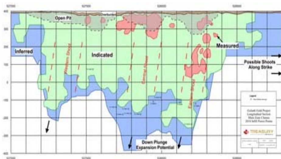
Figure 2: Main Zone Long Section
