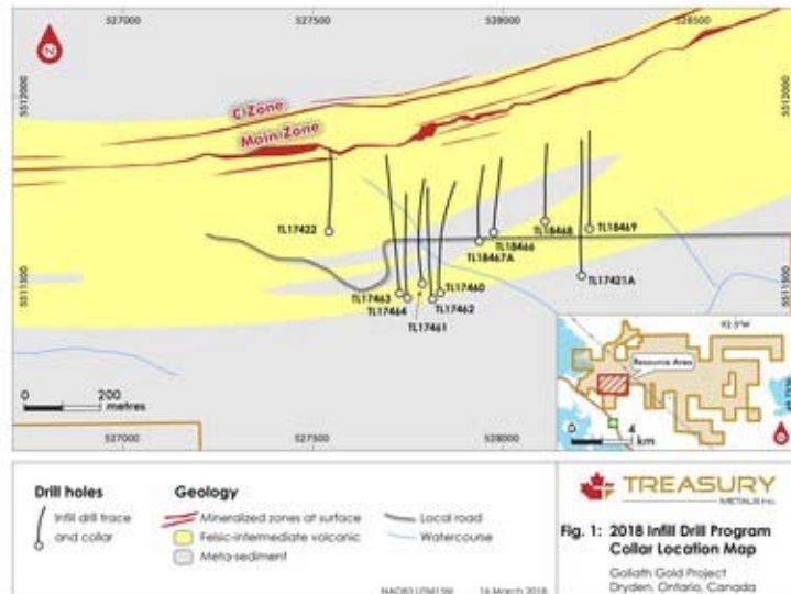
Figure 1: 2018 Infill Drill Program Collar Location Map
