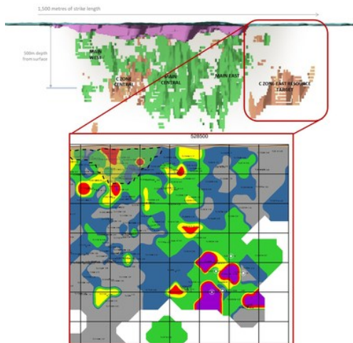
Figure 2: Goliath Gold Project C Zone Longitudinal Section of the Developing East C Zone Shoot. The updated Main Zone Longitudinal Section is available on the website. (CNW Group/Treasury Metals Inc.)
