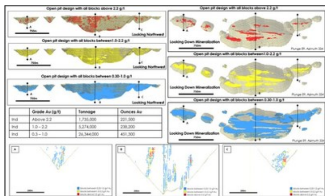
Figure 3: Goldlund Open Pit Resource with Block Model grade intervals. The top three images on the left side of Figure 3 are long section view looking Northwest. The top three images on the right side of Figure 1 are looking down the plunge of mineralization at Goliath and have been rotated ~30 degrees from looking straight down on the deposit. The underground cut-off grade is 2.2 g/t Au. (CNW Group/Treasury Metals Inc.)
