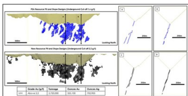
Figure 2: Goliath Underground Mineral Resource. The top figures represent the open pit and underground designs for PEA MRE. The bottom figure represents the open pit and underground designs for the updated MRE. The images on the left are looking North, and the other images are cross-section examples. (CNW Group/Treasury Metals Inc.)
