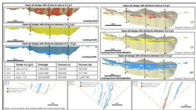
Figure 1: Goliath Open Pit Mineral Resource with Block Model grade intervals. The top three images on the left side of Figure 1 are long section view looking North. The top three images on the right side of Figure 1 are looking down the plunge of mineralization at Goliath and have been rotated ~30 degrees from looking straight down on the deposit. The underground cut-off grade is 2.2 g/t Au. (CNW Group/Treasury Metals Inc.)
