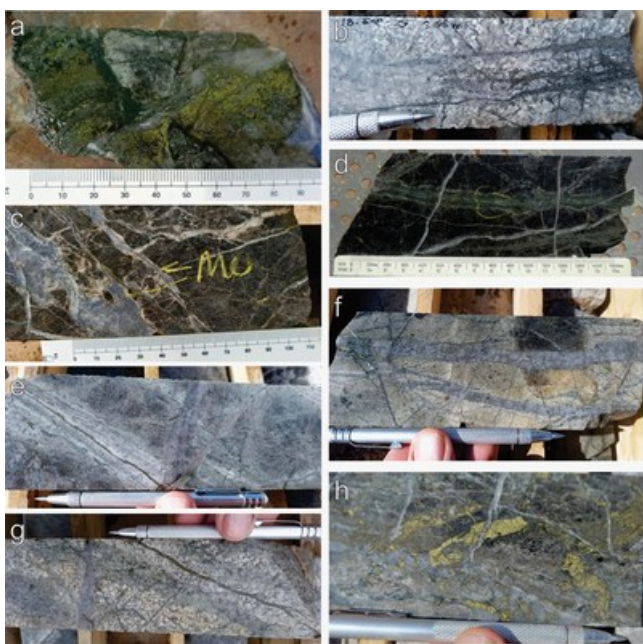
Figure 1: Textural examples of mineralization and alteration styles in Esperanza drill hole 18-ESP-25: (a) chlorite-green sericite -chalcopyrite + late gypsum veinlets, (b) "D" type pyrite-bornite-calcite veinlets with white sericite halo, (c) molybdenite in gypsum veinlets with strong pervasive secondary biotite and K-feldspar flooding, (d) chalcopyrite>pyrite veinlets with chlorite-green sericite haloes, cut by late gypsum veinlets, (e) "A" type veinlet, chalcopyrite-chlorite-green sericite, cut by "D" vein pyrite-bornite with white sericite halo, (f) stockwork of "A" type veinlets, host altered by intense K-feldspar flooding, cut by hairline chalcopyrite-pyrite-chlorite veinlets, (g) "A" type veinlets with chalcopyrite-chlorite-green sericite, cut by "D" type pyrite-bornite veins with white sericite halo, (h) coarse chalcopyrite>pyrite-chlorite-green sericite veins with late gypsum veins. (CNW Group/Libero Copper & Gold Corporation.)
