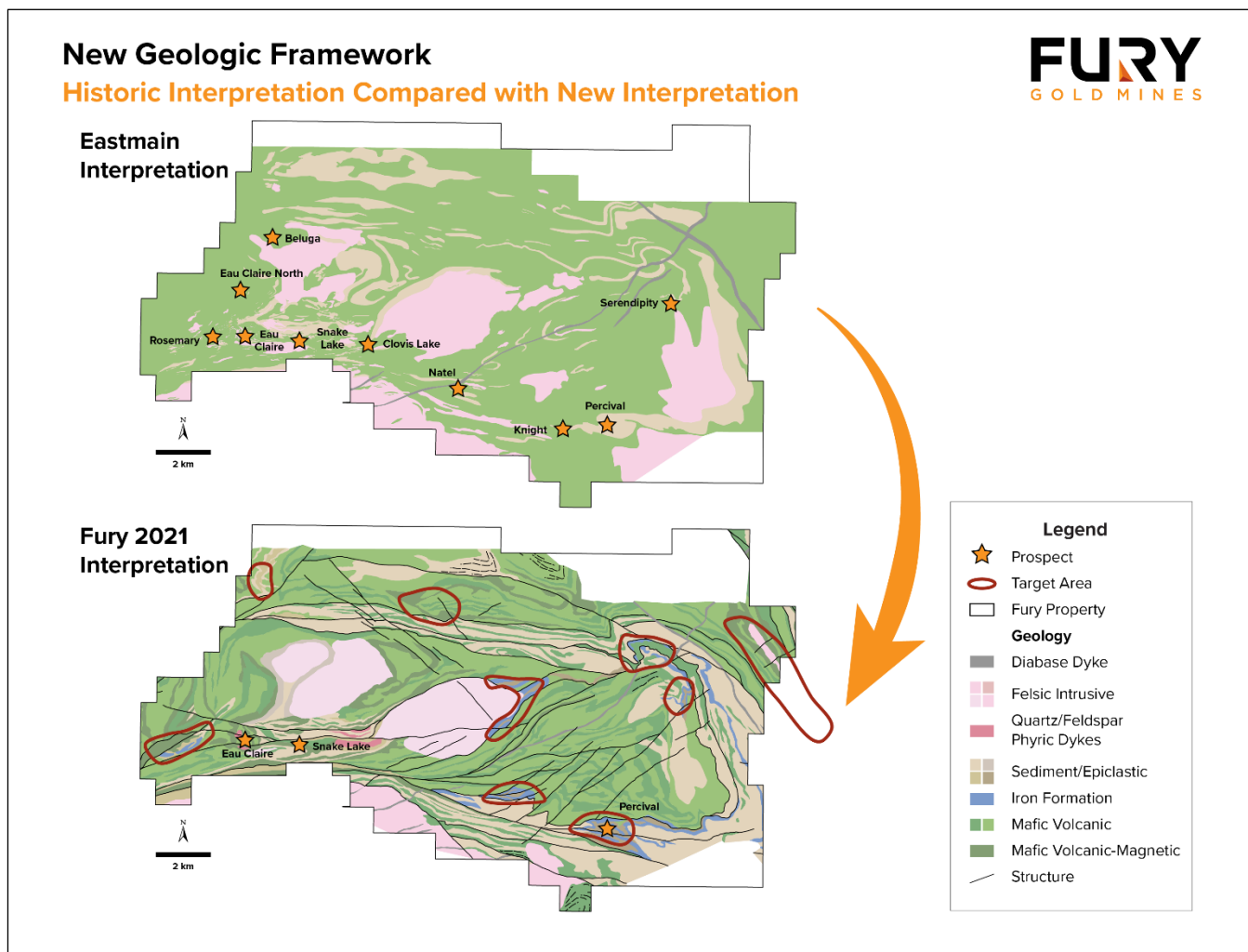
Figure 1: Updated Geologic Framework compared with the historical interpretation at Eau Claire.
