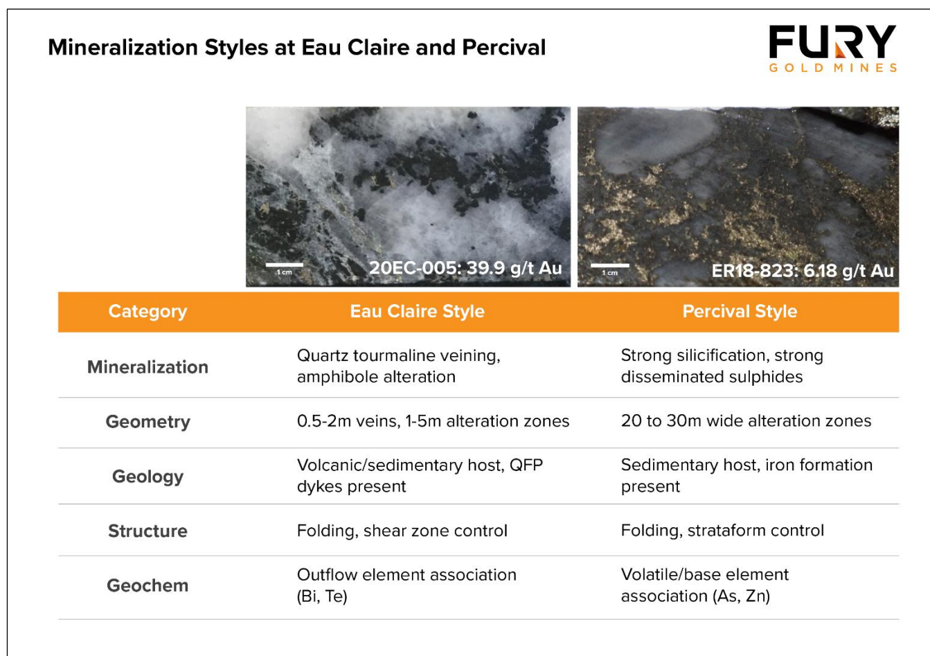
Figure 2: Comparison of the two principal styles of mineralization present at Eau Claire.
