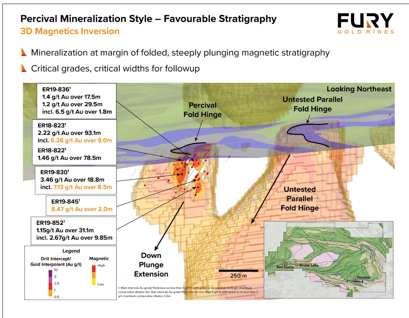
Figure 3: New interpretation of the Percival prospect showing the steep west fold plunge as indicated by the 3D magnetic inversion.
