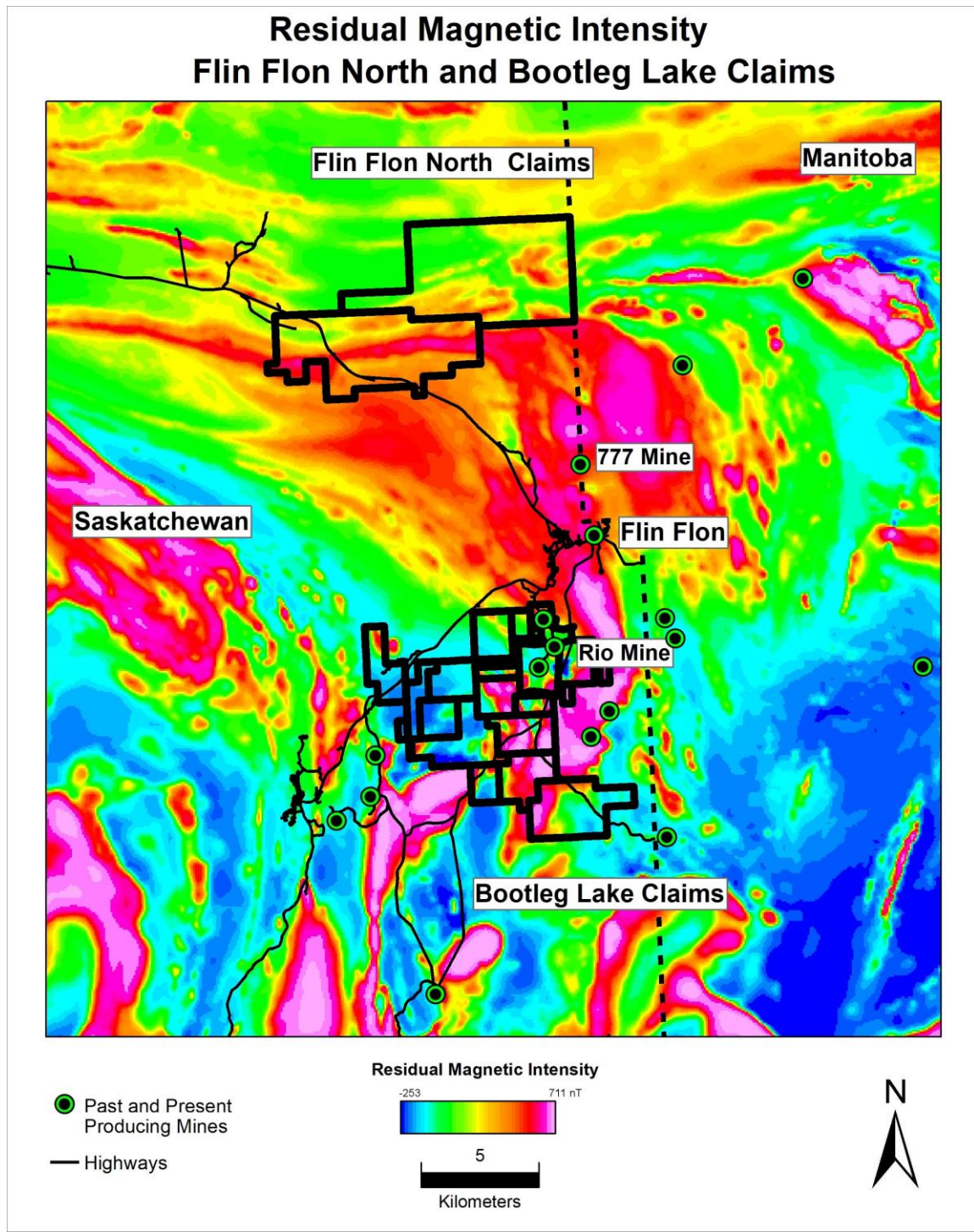
Figure 2 Residual Magnetic Intensity Flin Flon Claims.
