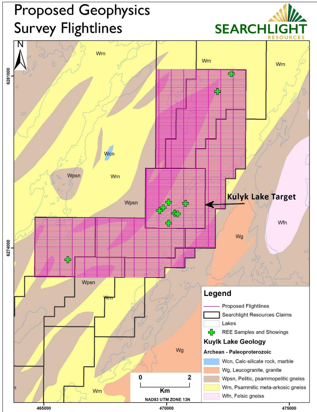
Map 1. Proposed flightlines for aeromagnetic and radiometric surveys over Kulyk Lake Property
