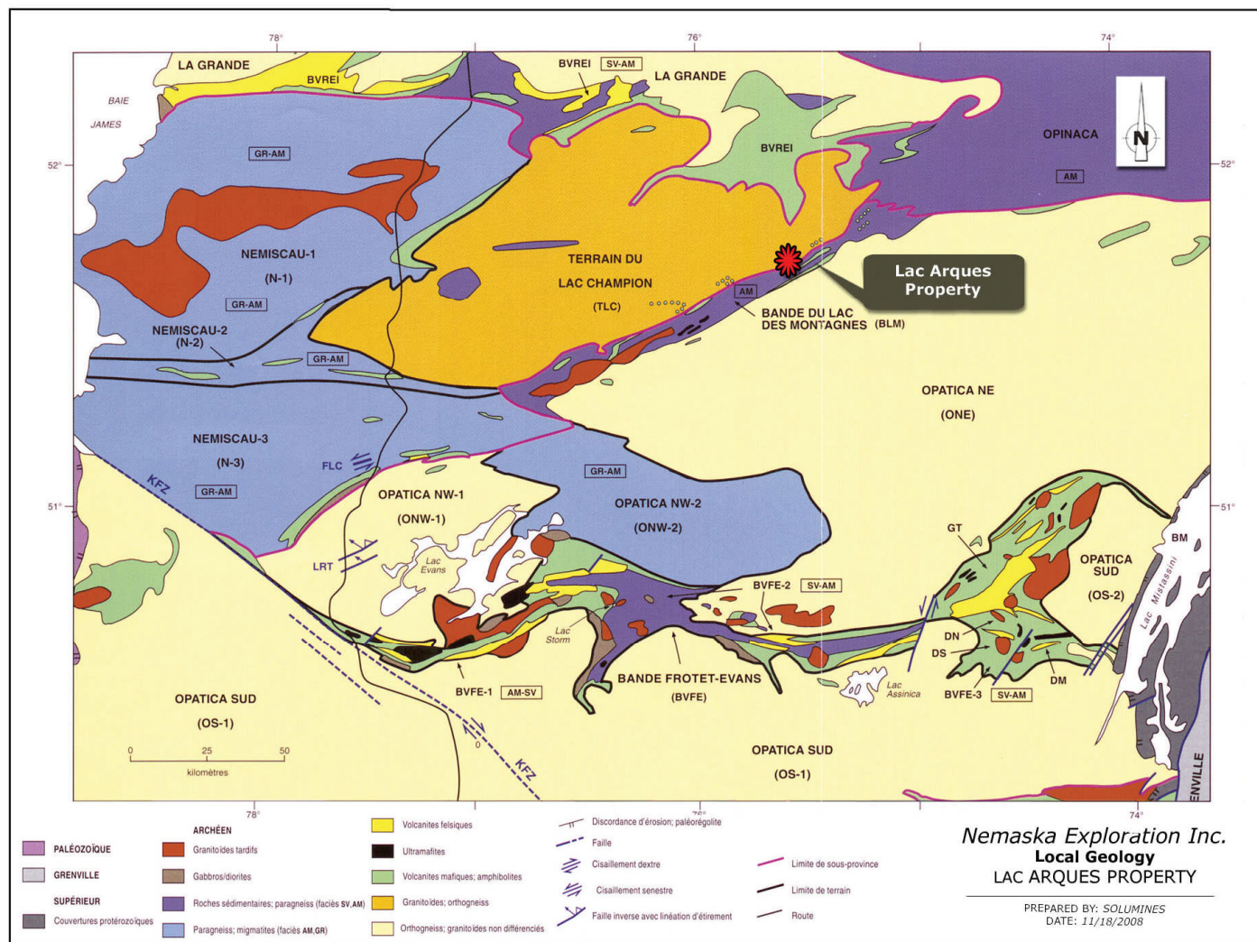
Figure 5: Local Geology
