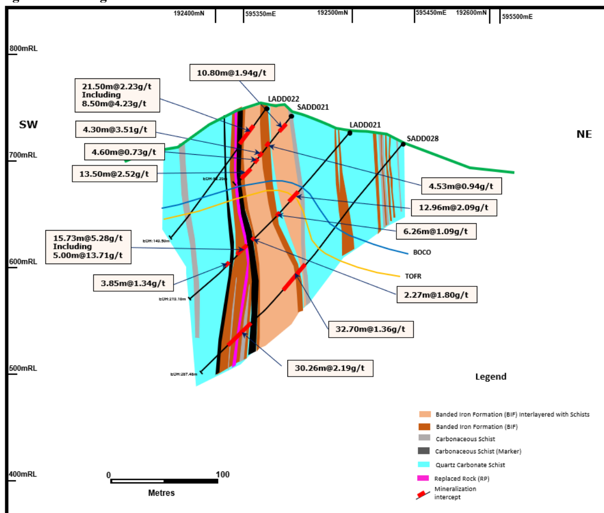
Figure 2: Geological Cross Section A-B
