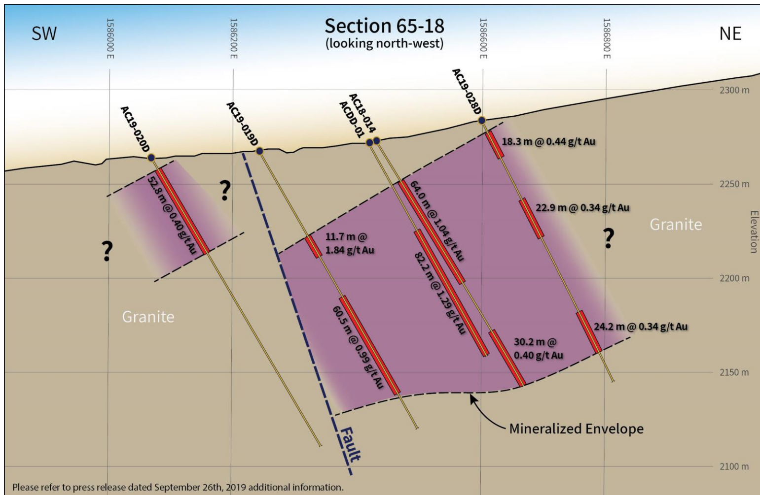
Figure 2 – Preliminary Arnett Haidee Cross-Sectional Interpretation (September 26 th , 2019)
