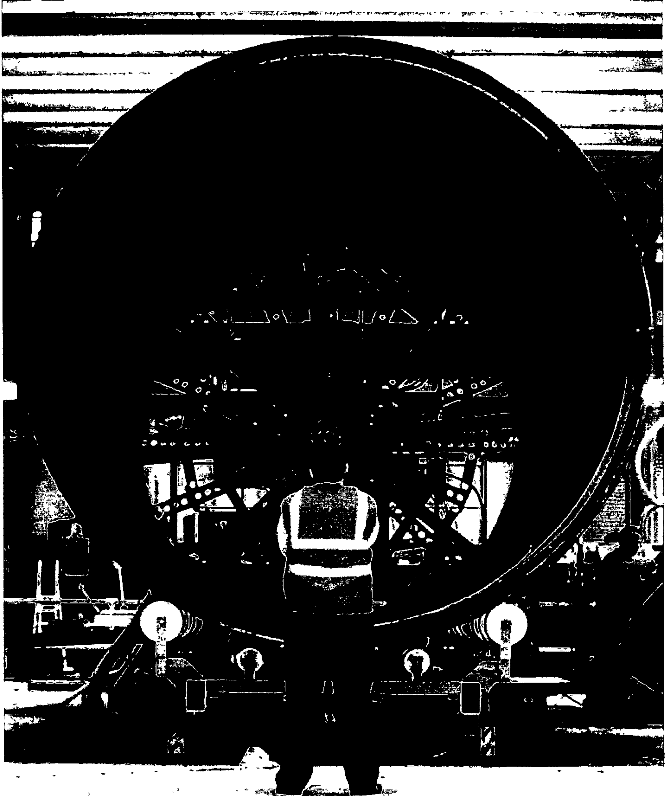
Asset Weholite HDPE production line manufacturing the largest plastic pipe in the world (3.5m diameter) for the AMP5 market
