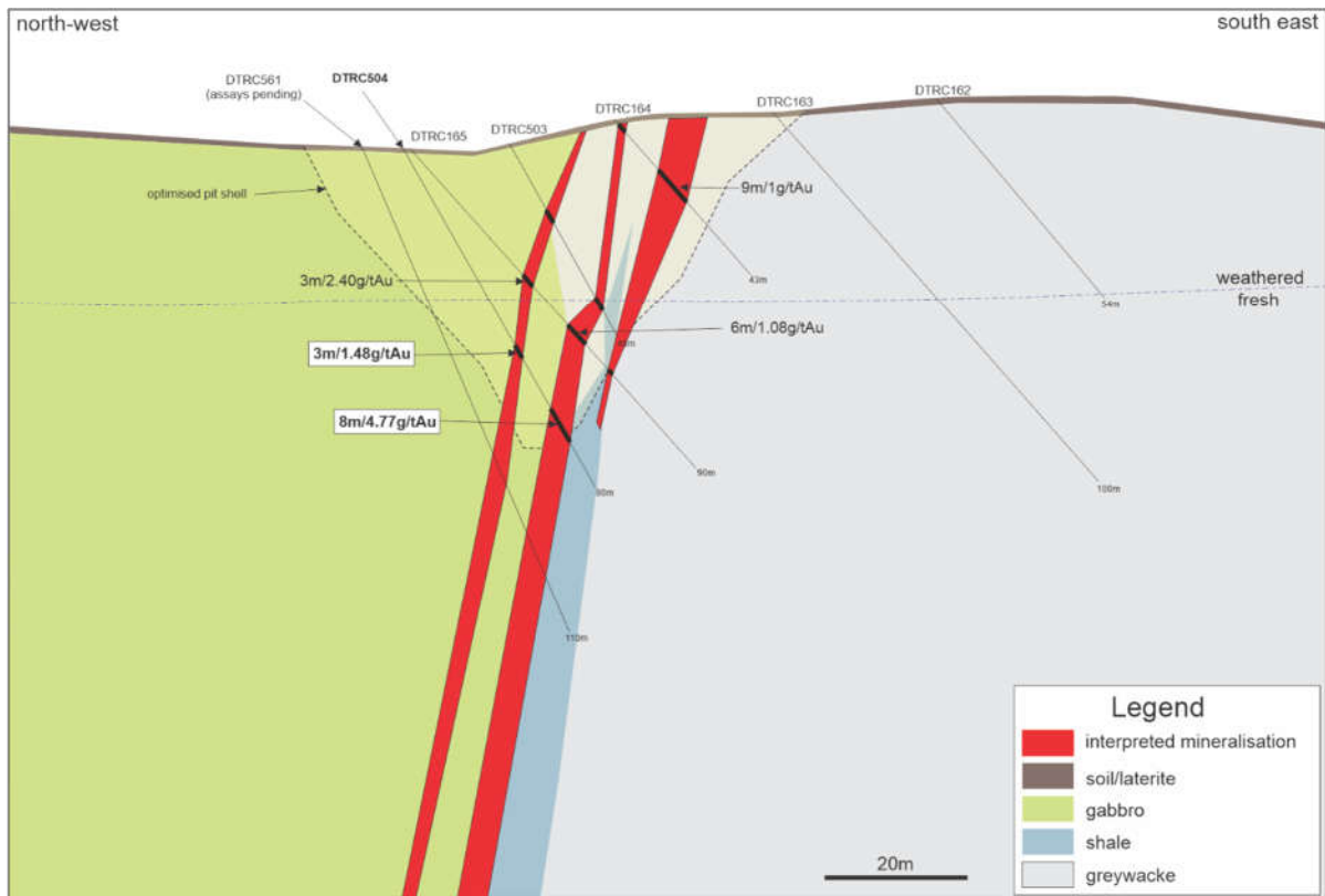
Figure 7: Makosa Cross Section
