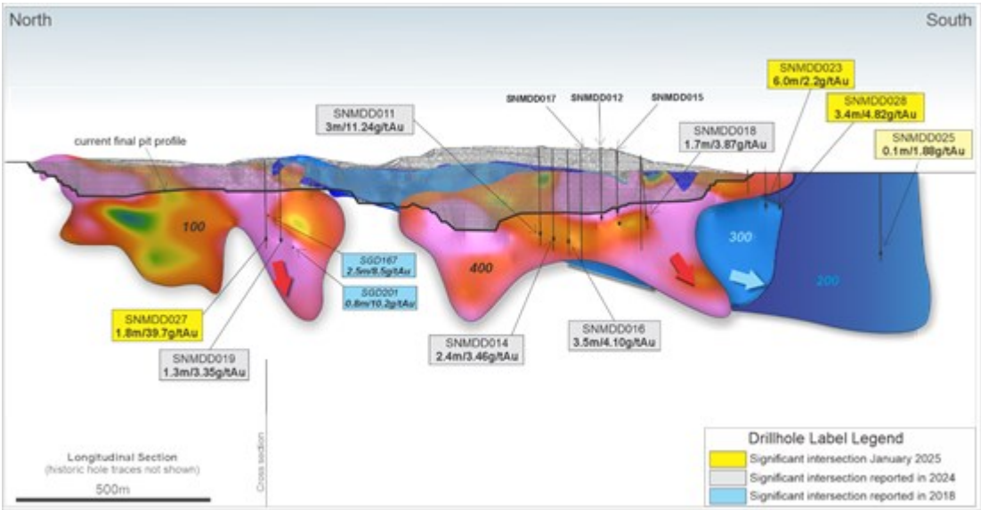
Figure 1: Longitudinal Section Showing Drilling Results
