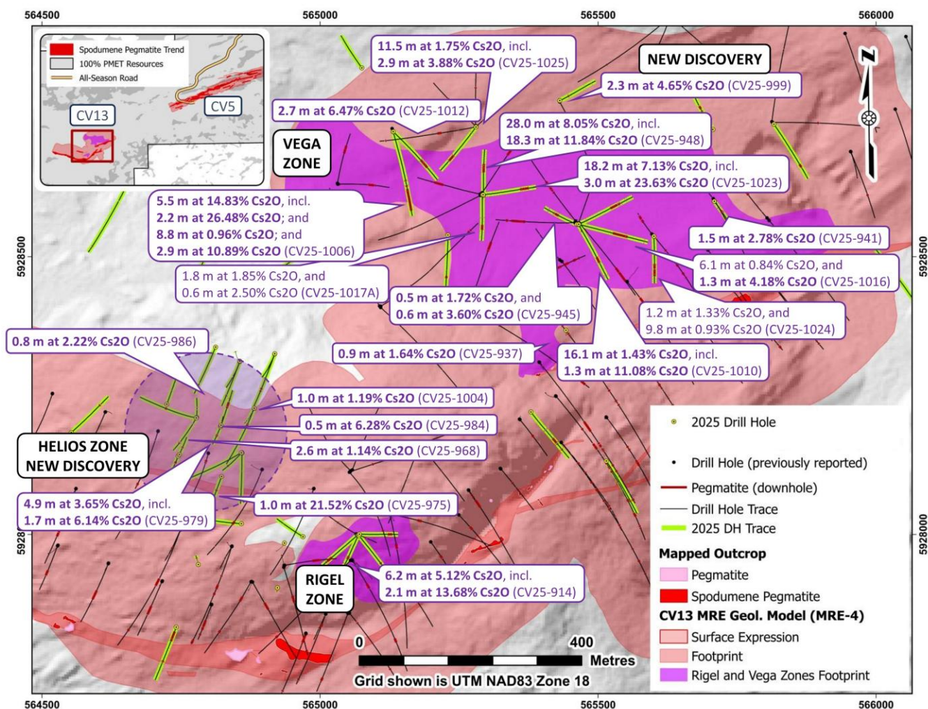
Figure 2: Drill hole result highlights at the CV13 Pegmatite (caesium).
