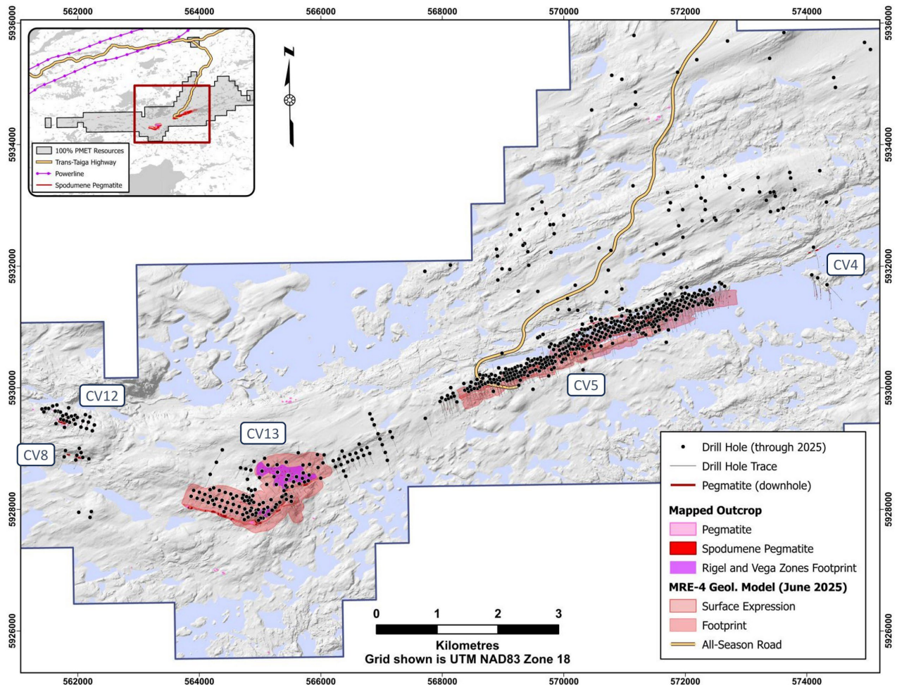
Figure 1: Location of the principal corridor at Shaakichiuwaanaan, which is host to the CV5 and CV13 LCT pegmatites.
