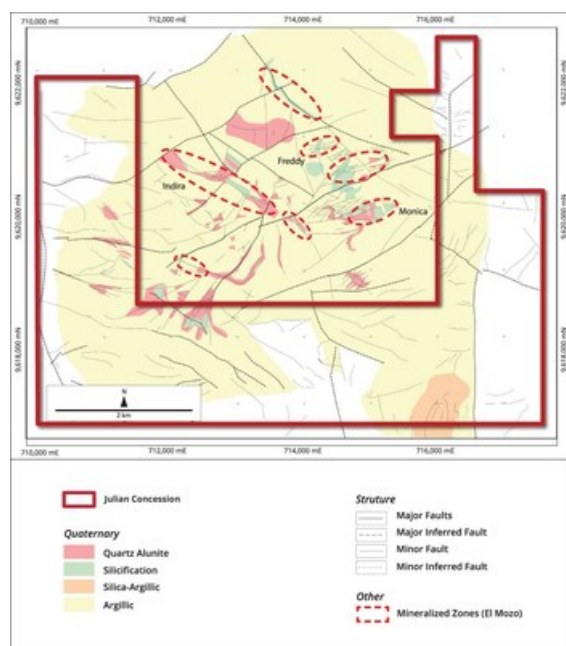
Figure 1: Alteration map of the Property and the adjacent El Mozo high-sulphidation epithermal gold deposit. Known gold mineralization at El Mozo is shown. (From Julian NI43-101 Technical Report, March 31, 2020) (CNW Group/Oro X Mining Corp.)
