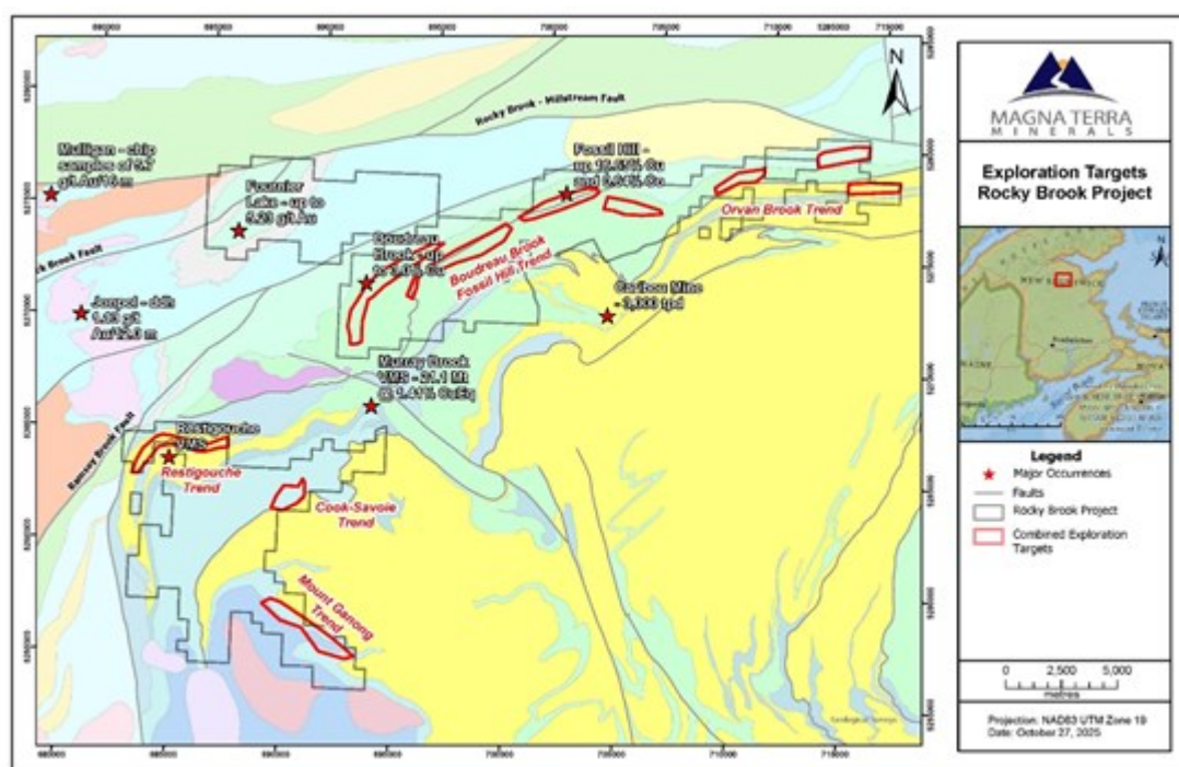
Figure 1: A map showing the location of the Rocky Brook Project, regional geology and major target areas generated in the current Windfall and Mira studies.
