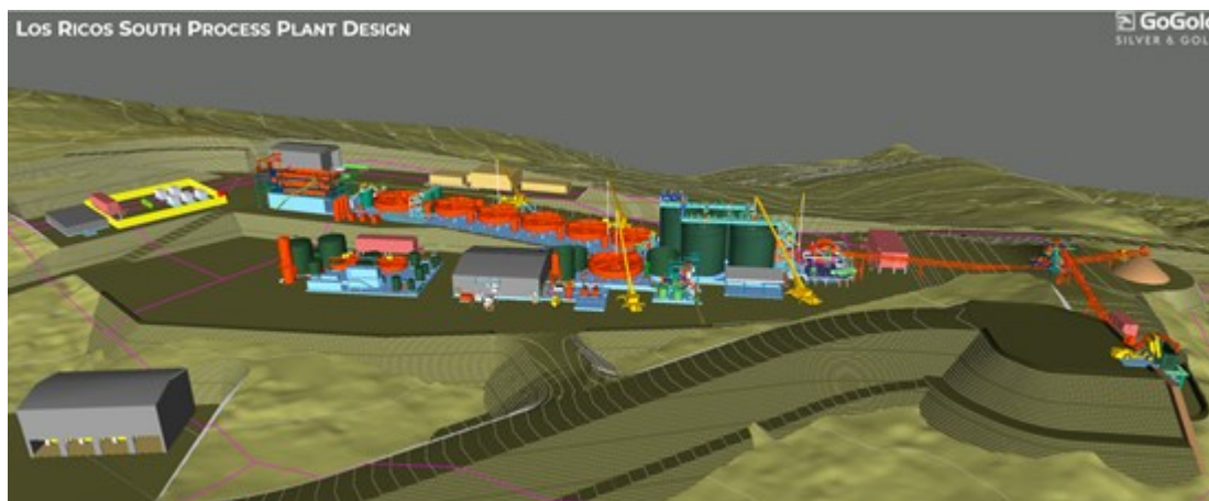
Figure 5 - Process Plant Design
