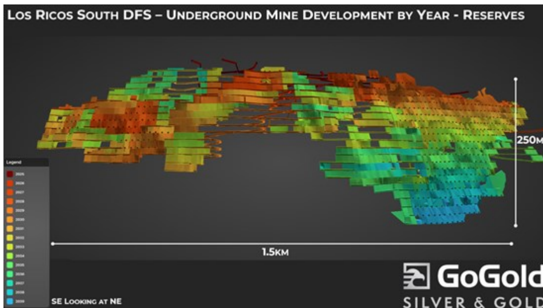
Figure 4 - Underground Mine Plan by Year
