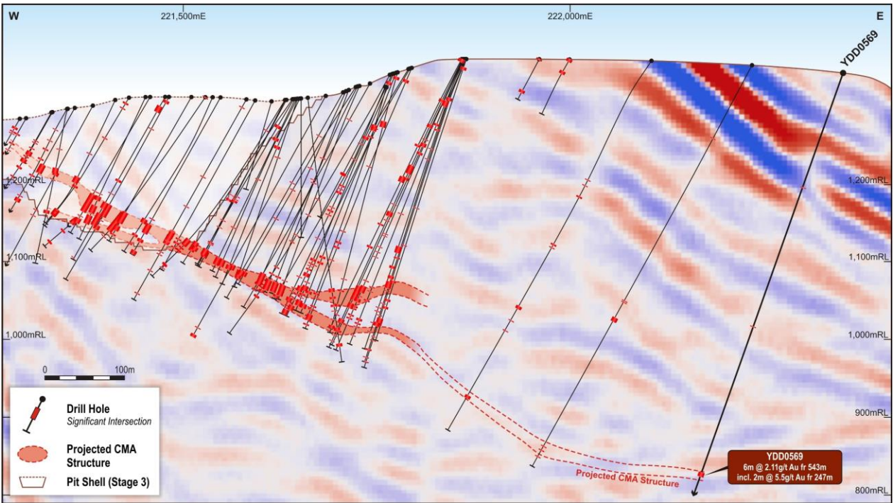
Figure 5: CMA Deep Drilling Section - Drill Section 776,975mN (+/- 50m window)
