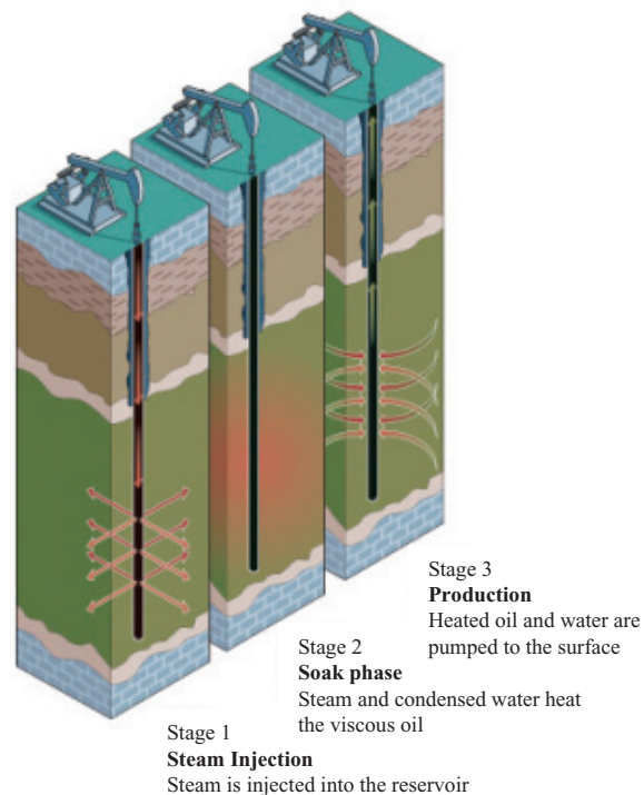
Cyclic Steam Stimulation (CSS) Process (1)
