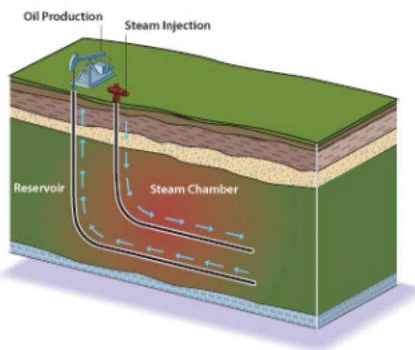
Steam Assisted Gravity Drainage (SAGD) Process (1)
