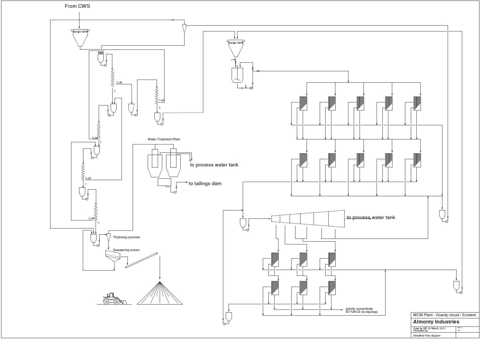
Figure 17-2. Overall Flowsheet
