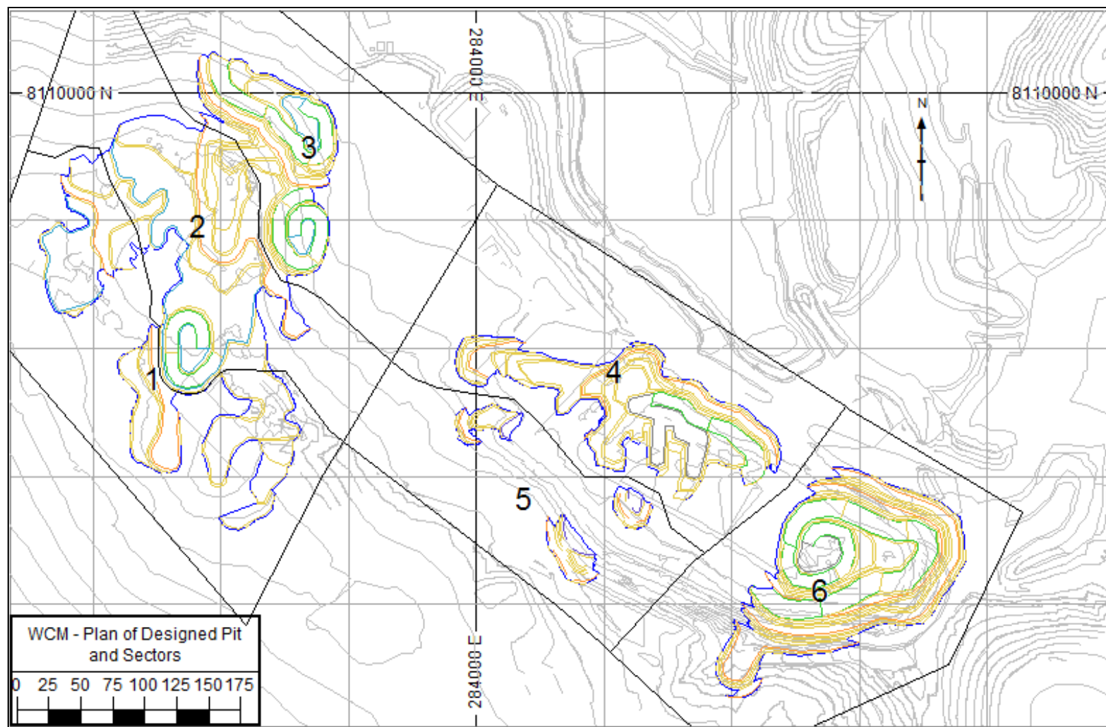
Figure 15-4. Plan of Design Pit and Sectors
