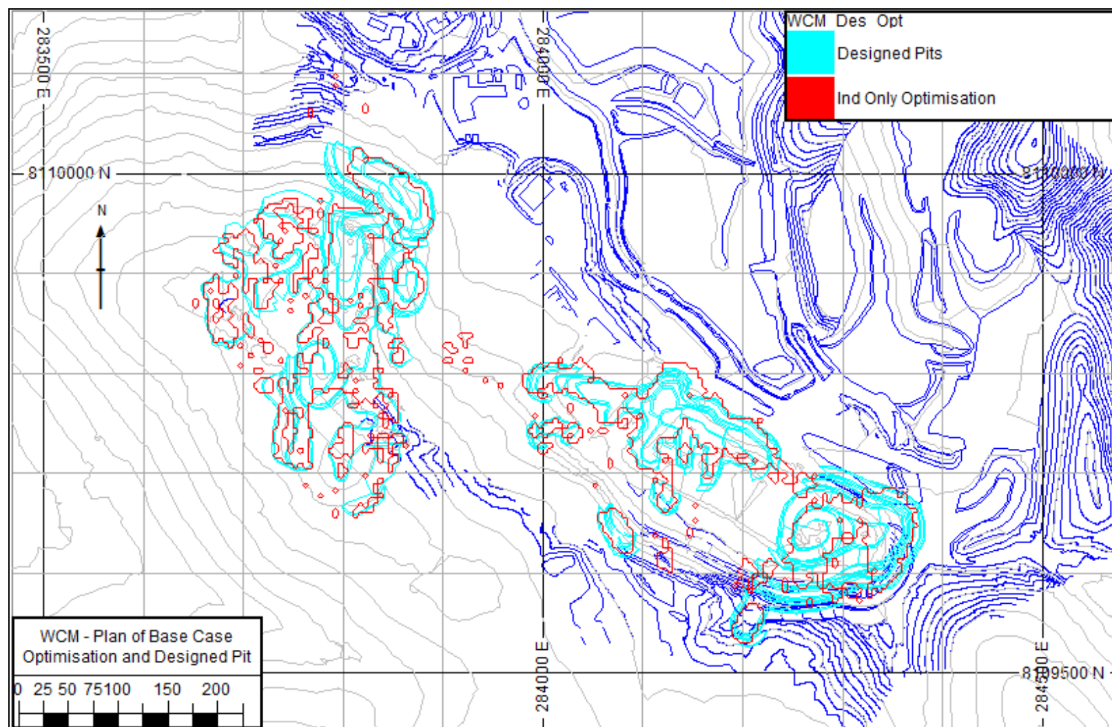
Figure 15-1. Plan of Base Case Optimal and Designed Pits
