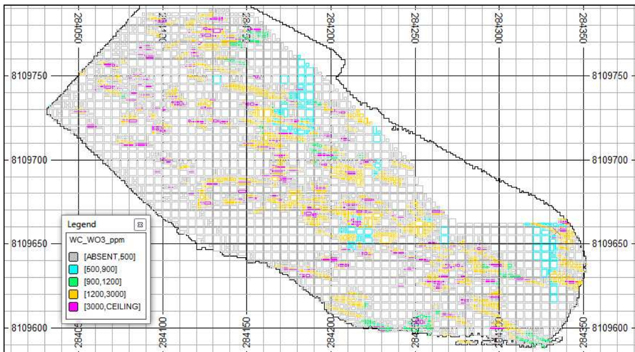
Figure 14-16. Plan at 573.25mRL - Test Evaluation Model, March 13- March 14 (Based only on DD and RC data)
