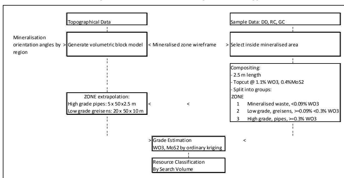
Figure 14-1. Block Modelling Methodology
