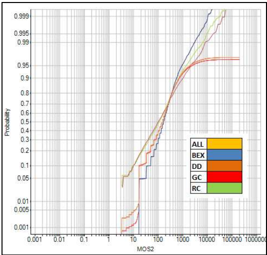
Figure 14-18. Log-Probability Plot, \text{MoS}_2 , Selected Samples
