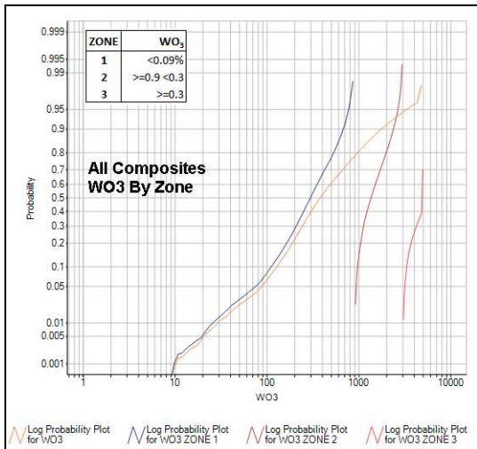
Figure 14-22. Log-Probability Plot, WO 3 – Composites by ZONE
