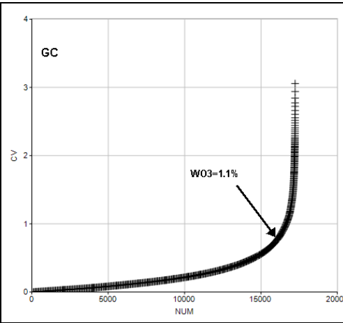
Figure 14-20. CV Analysis - GC Samples, \text{WO}_3
