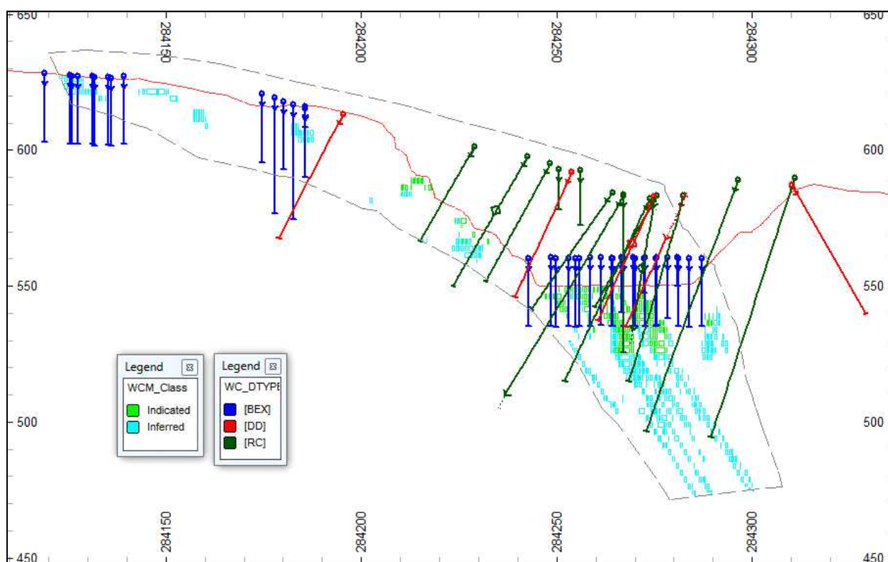
Figure 14-27. Example of Resource Classification – Section E-E'
