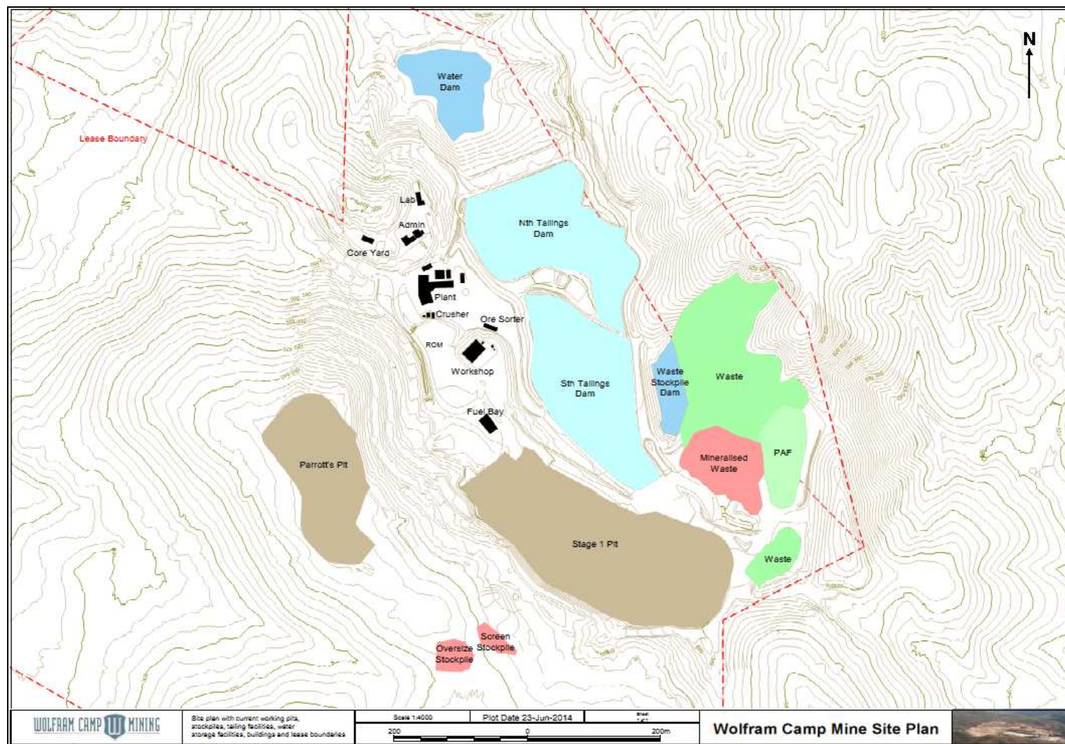
Figure 18-1. Site Plan
