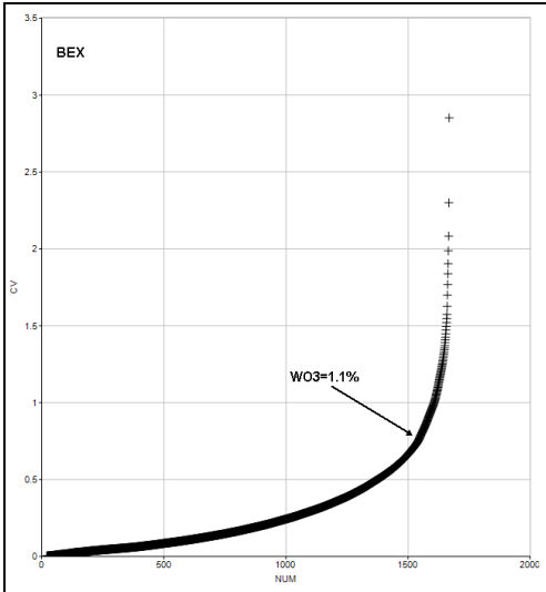
Figure 14-20. CV Analysis - GC Samples, \text{WO}_3
