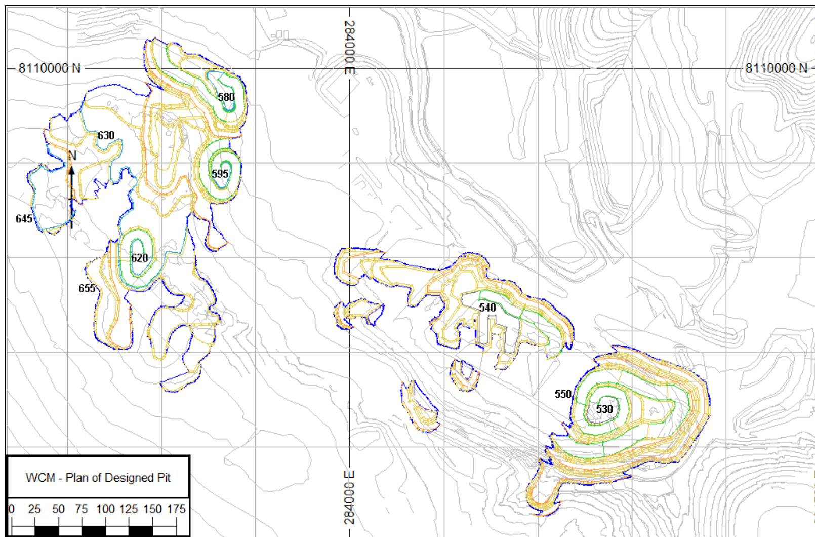
Figure 15-3. Plan of Pit Design
