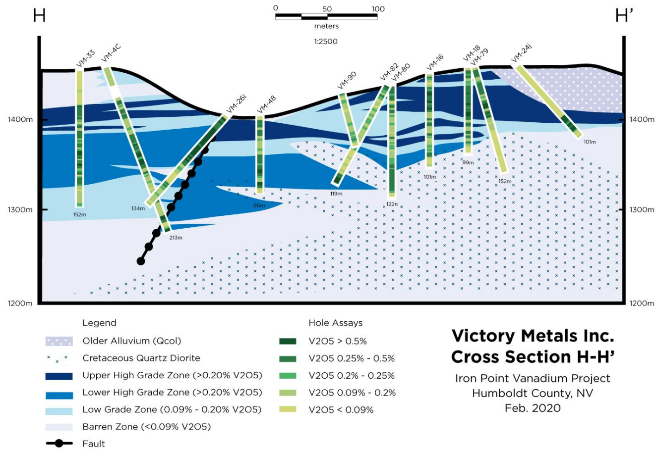
Figure 2. Cross section H-H' showing distribution of vanadium mineralization in relation to the current geologic interpretation.
