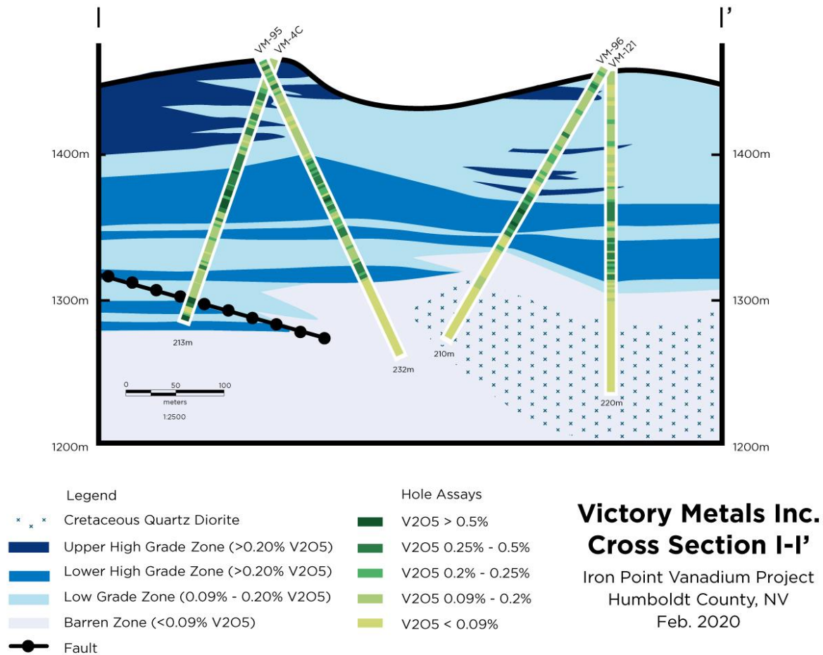
Figure 3. Cross section I-I' showing distribution of vanadium mineralization in relation to the current geologic interpretation.
