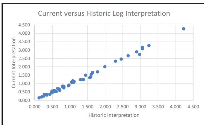
Figure 12.1 – Database Comparison
