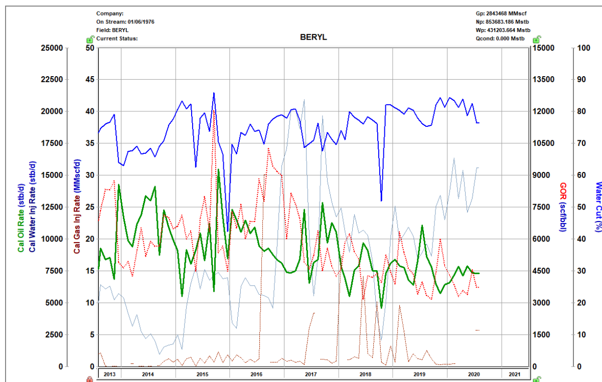
Figure 3-14: Beryl field recent production and injection history
