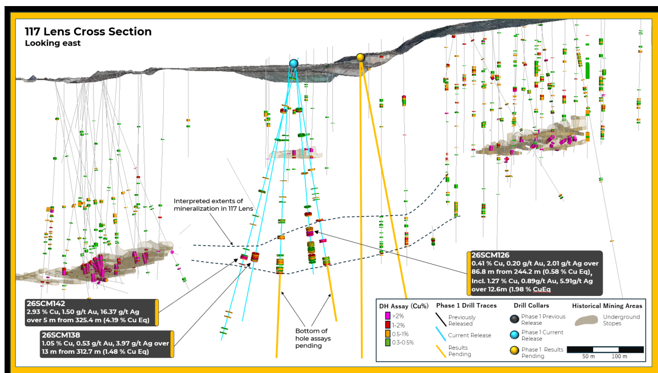
Figure 2: Cross section looking east, showing the recently discovered 117 Lens located beneath the Area 2 open pit and between two areas of previous underground mining.
